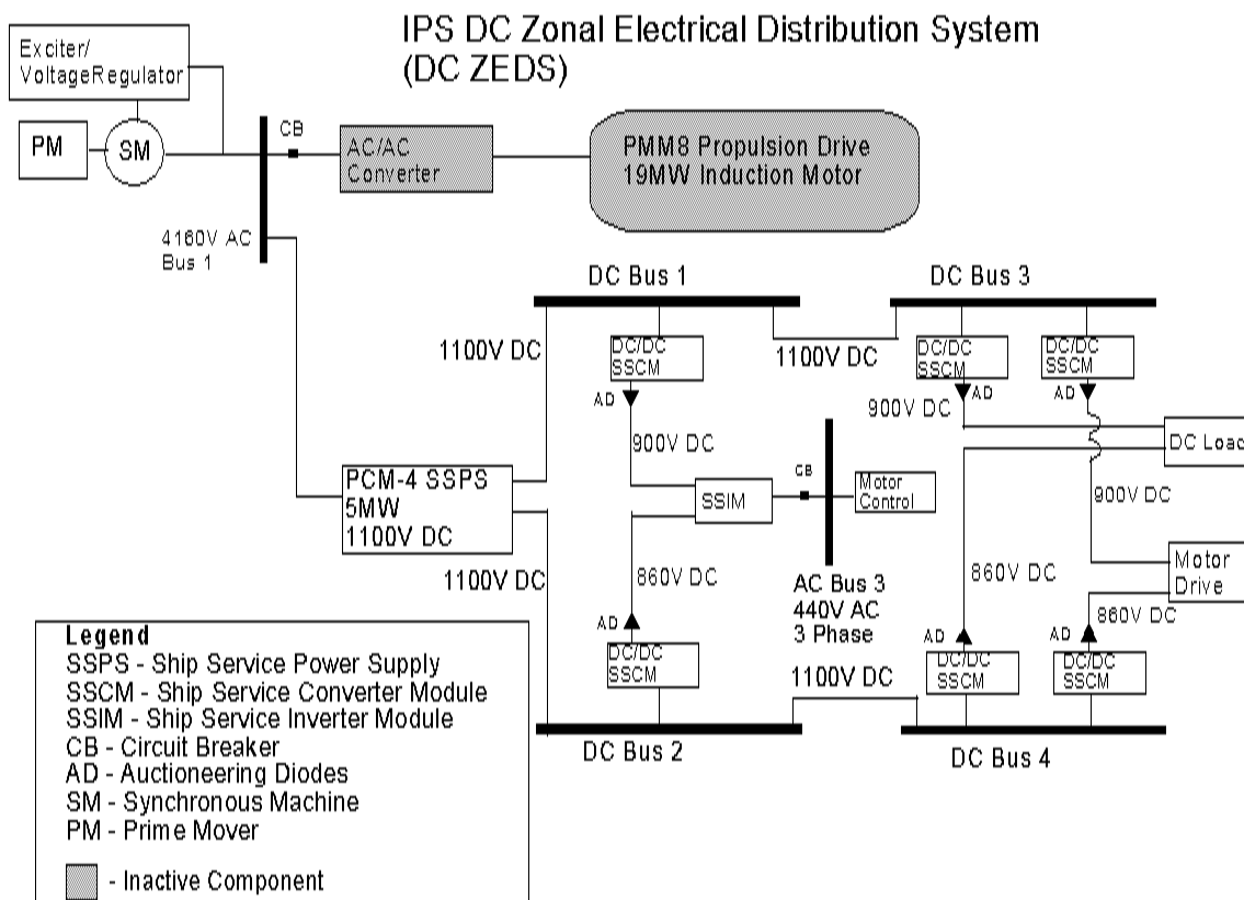
Figure 5-8 Run 6 Configuration
