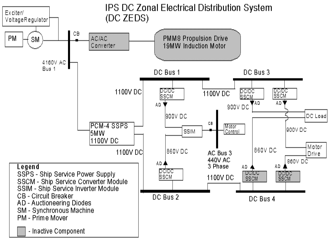
Figure 5-9 Run 7 Configuration
