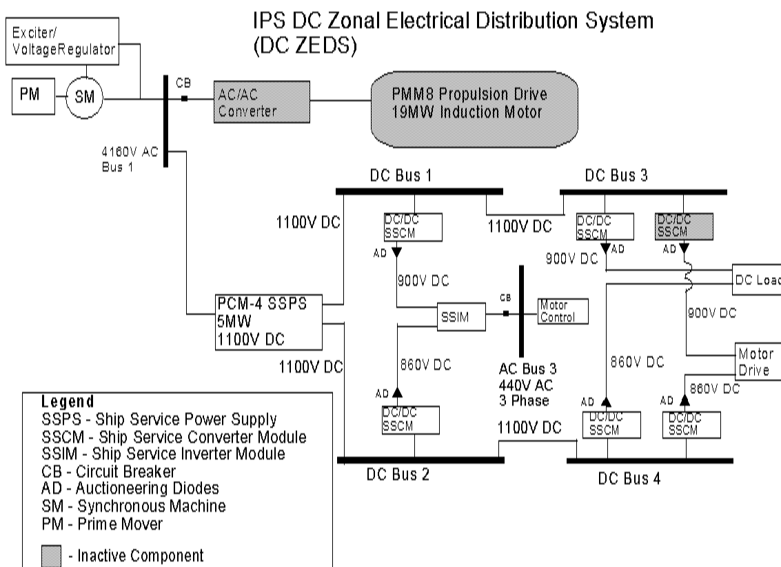
Figure 5-7 Run 5 Configuration
