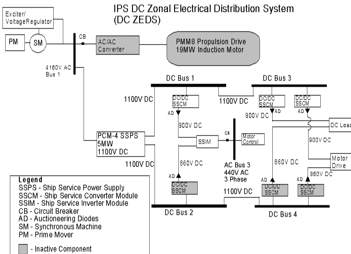
Figure 5-10 Run 8 Configuration
