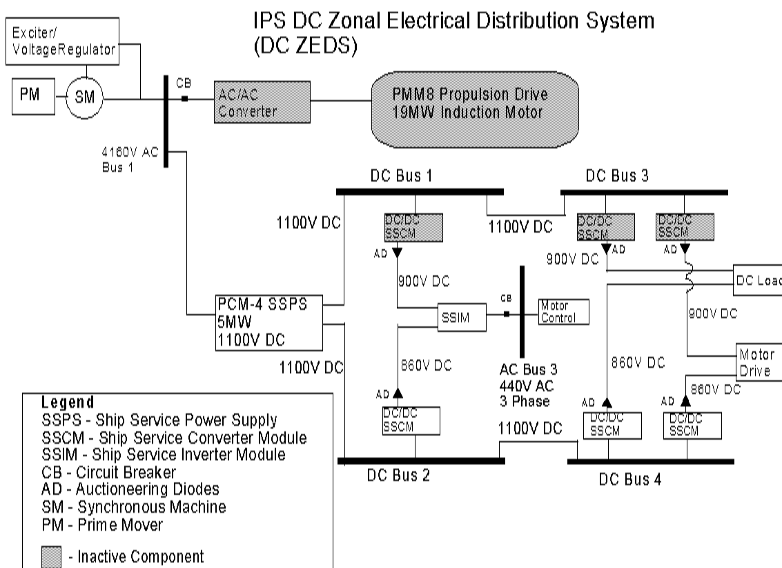
Figure 5-5 Run 3 Configuration
