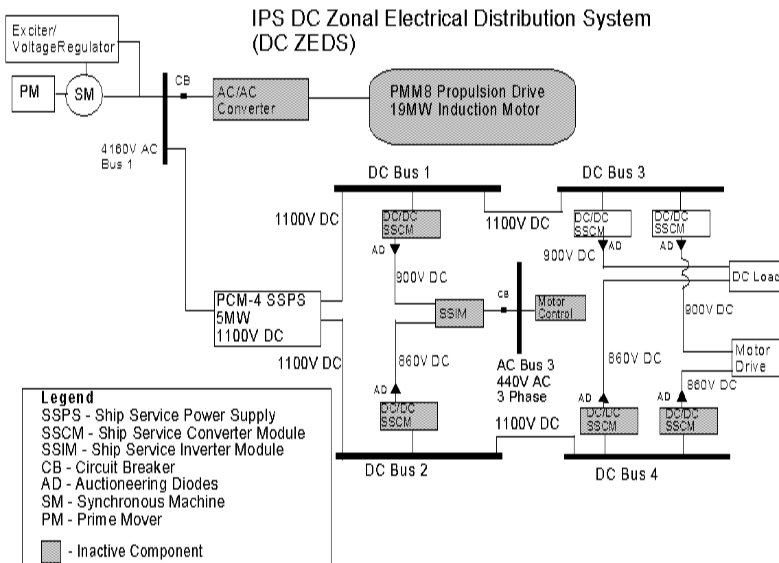
Figure 5-3 Run 1 Configuration
