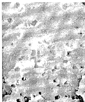
Photo 14: 2091. Fracture planes (110)
