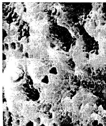
Photo 13: 2195. Fracture planes (111)
