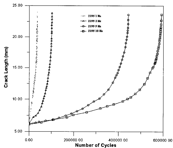
Figure 7: 2195 alloy
