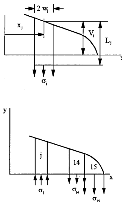
Figure 2: Elements and applied stresses
