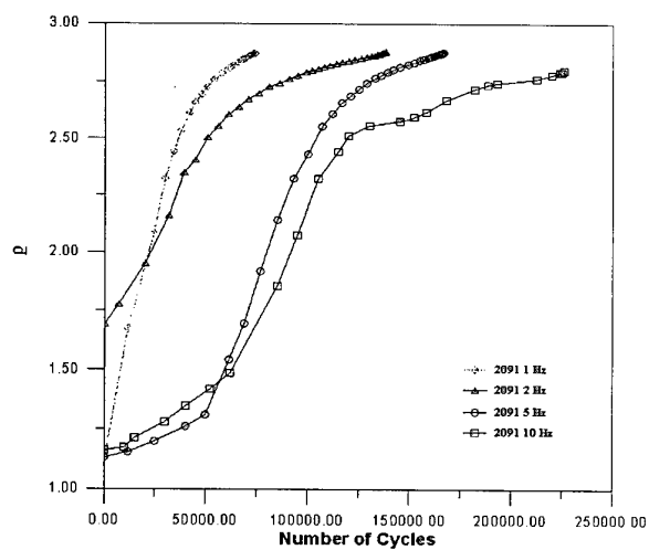
Figure 10: 2091 alloy
