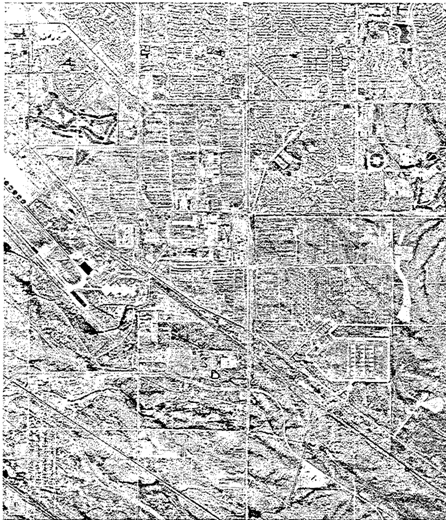
Figure 4.1: Aerial Photograph of Davis-Monthan Collect Area.
