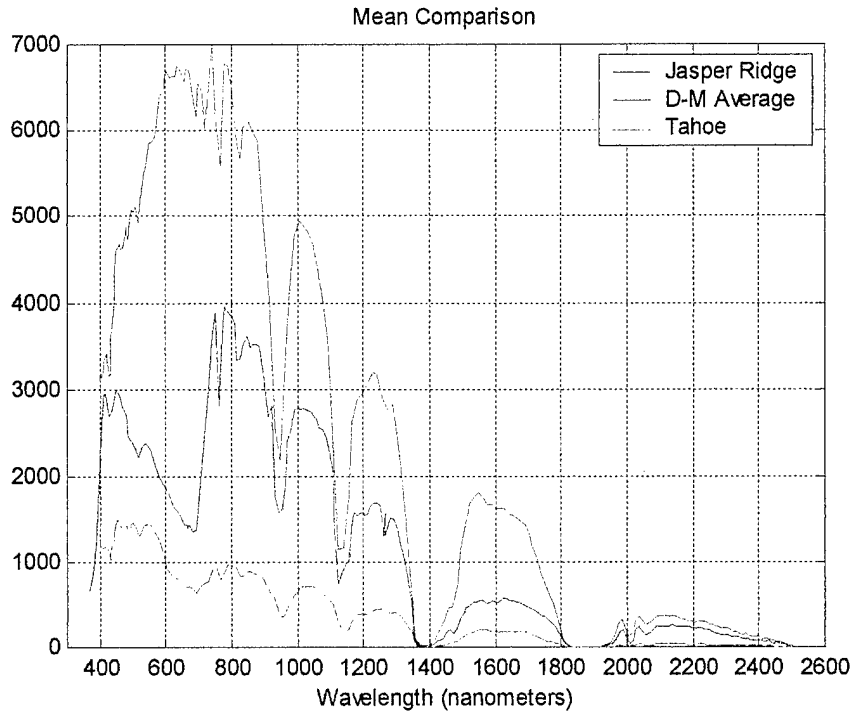
Figure 4.13: Jasper Ridge and Lake Tahoe Mean Compared to Davis-Monthan Average.
