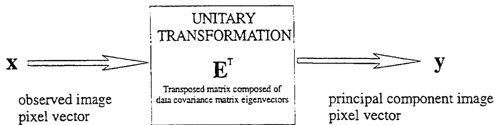
Figure 2.12: PC Transformation Depicted as a Linear Transformation.
