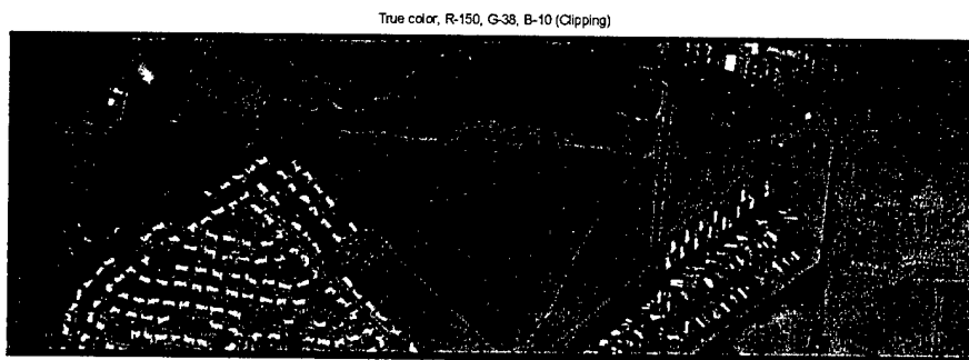
Figure 3.10: RGB Image with Original Data Bands 150, 38 and 10.
