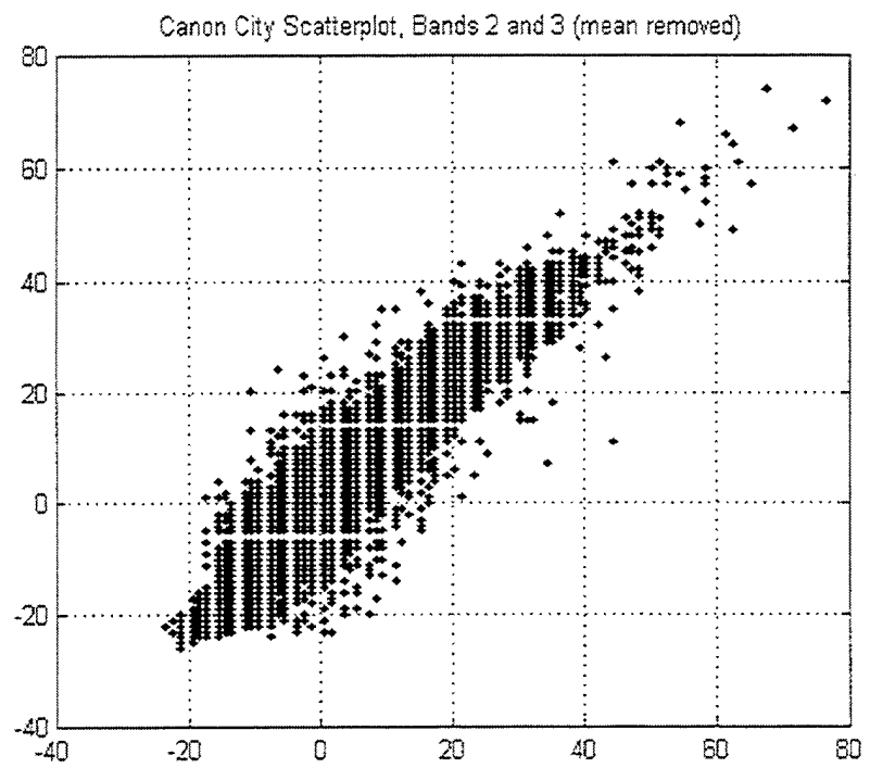
Figure 2.6: Mean Removal Illustration With Scatter Plots.
