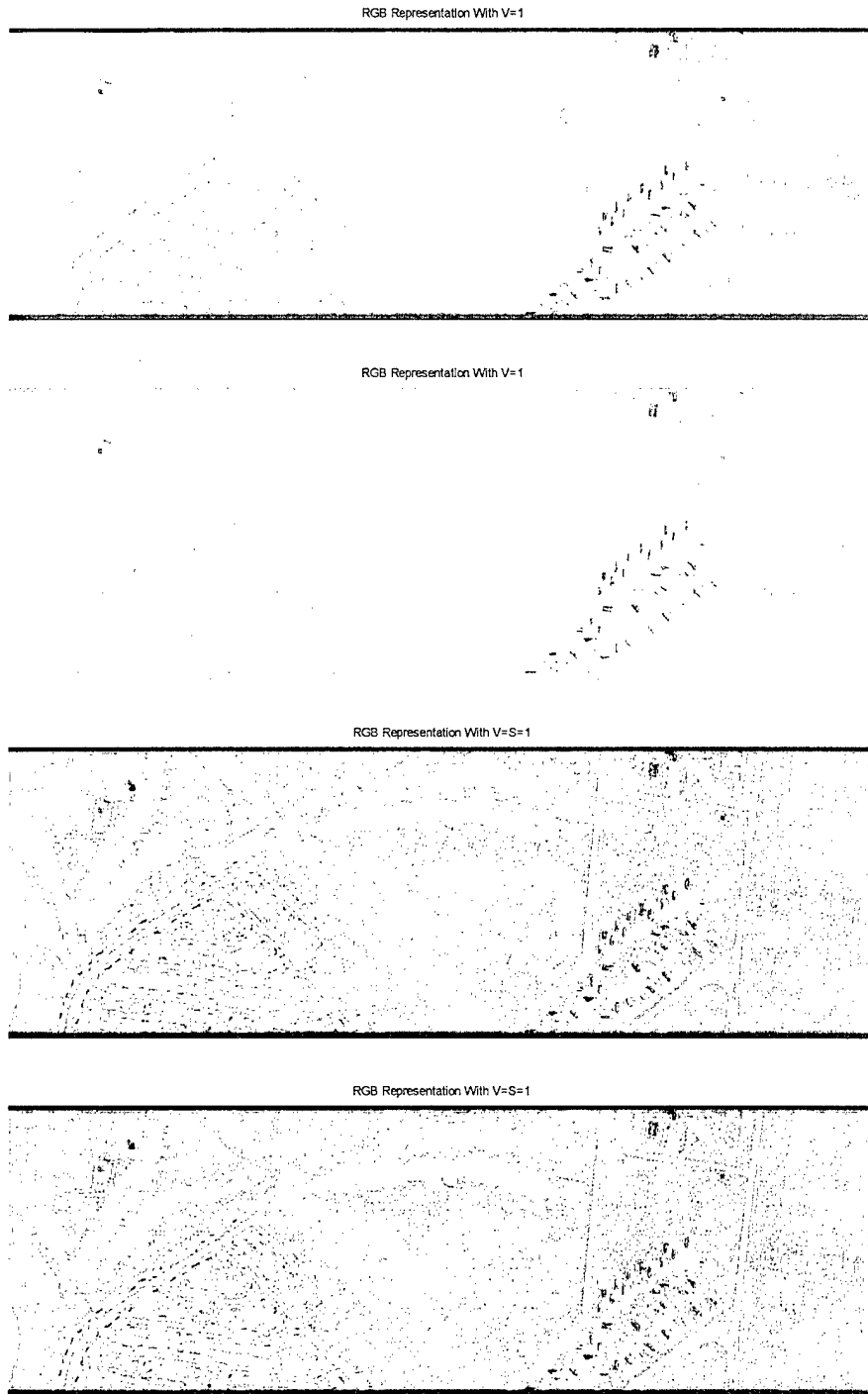
Figure 4.18b: Davis-Monthan Direct RGB Representation of Original PCs and Test PCs. Panels A and C are from the Original Data. Panels B and D are from the Test Set. (Note the similarity between panels A and B, and C and D.)
