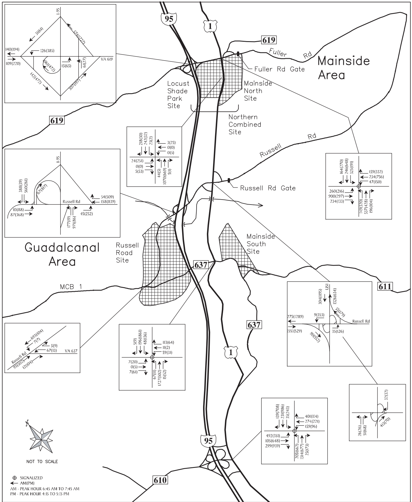
Figure 4-10 Northern Combined Site Total Peak Hour Volume (2015)
