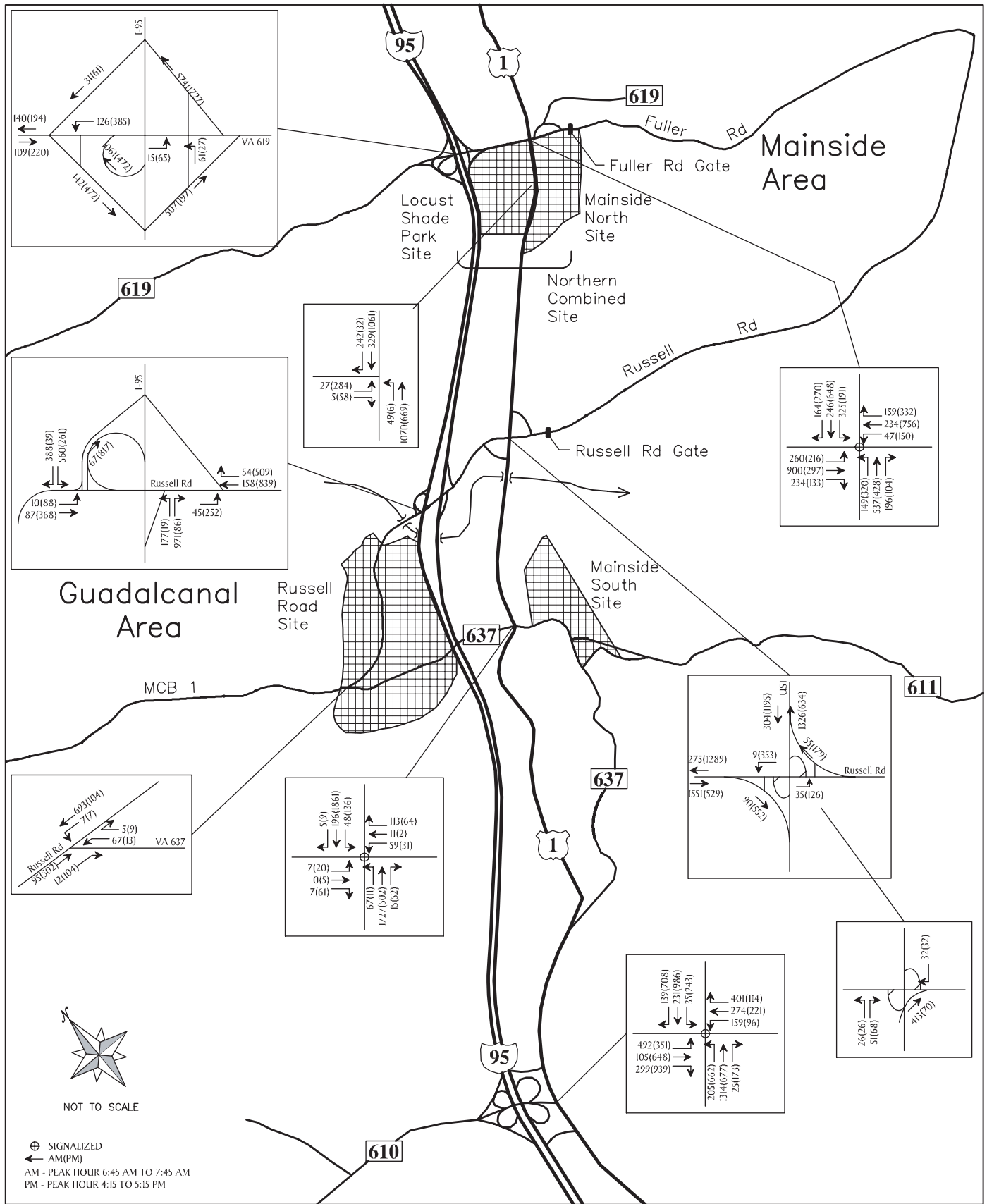
Figure 4-9 Locust Shade Park Site Total Peak Hour Volume (2015)
