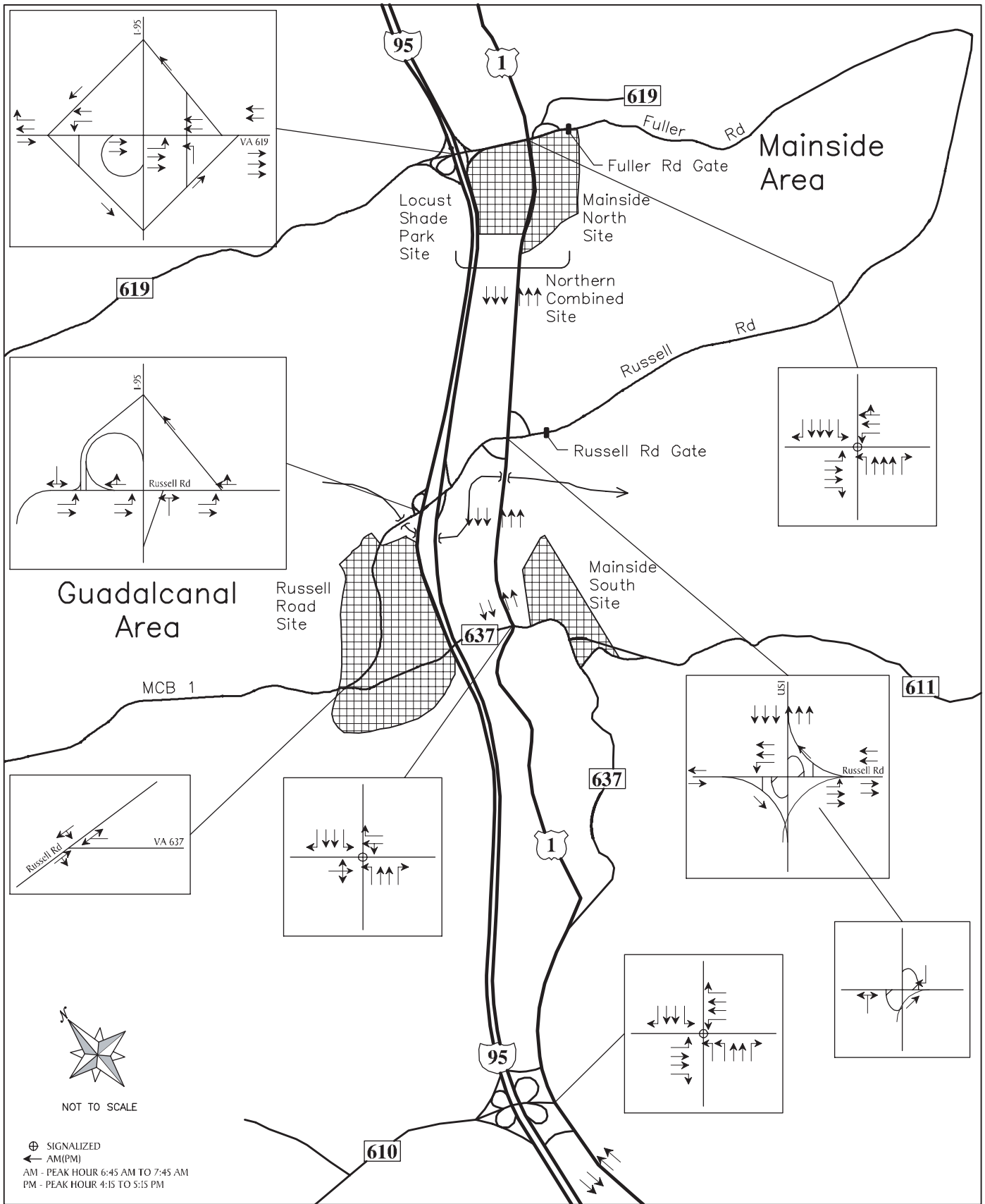
Figure 3-21 Background Lane Uses
