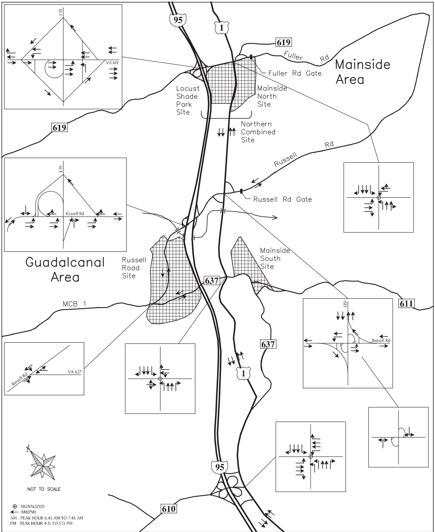
Figure 3-19 Existing Road and Lane Uses
