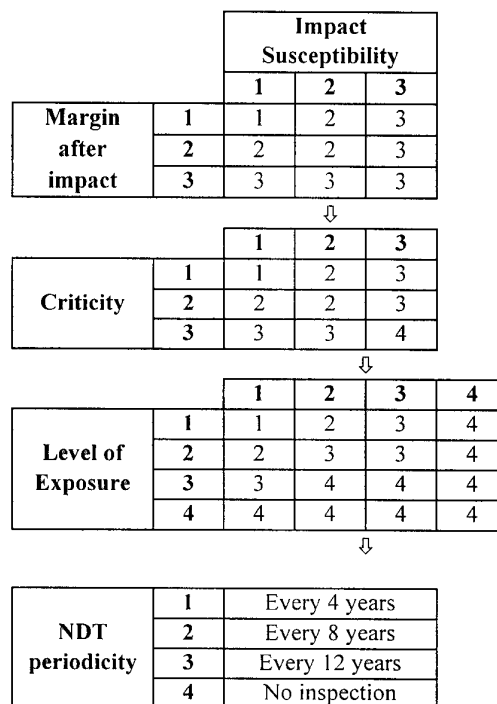
Figure 4 : Selection grid for impact damage
