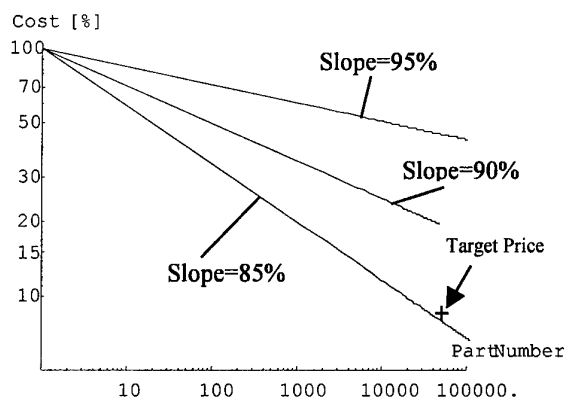
Fig. 17: Learning curves for Manufacturing of Electronic Elements
