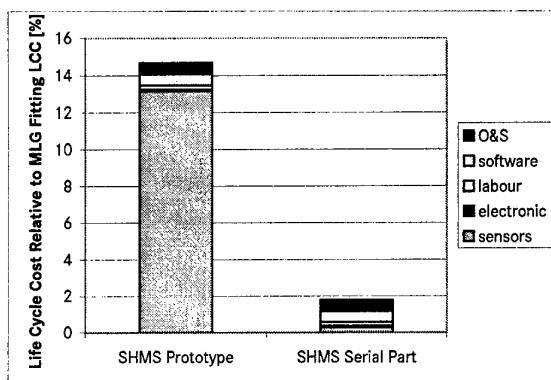
Fig. 16: Cost Structure of the SHMS Prototype and the Serial Part
