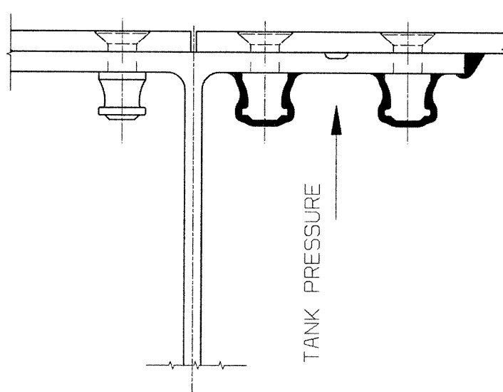
Fig. 3.6: Integral fuel tank sealing
