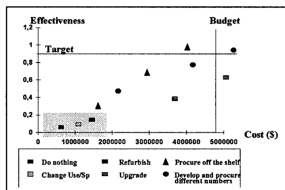
Figure 8: Cost-effectiveness for existing systems
