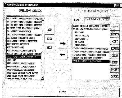
Figure 10 - Manufacturing Operation Sequence
