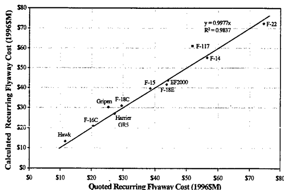
Figure 4. Recurring Flyaway Cost Comparison (FY96).
