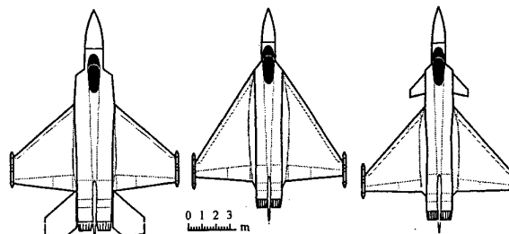
Figure 7. Twin-Engine Configuration Solutions.
