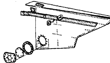
Fig. 9: Tail Section Skin
