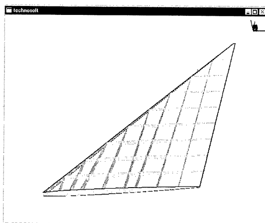
Figure 8 - AML geometry of a Wing Decomposed to Substructure
