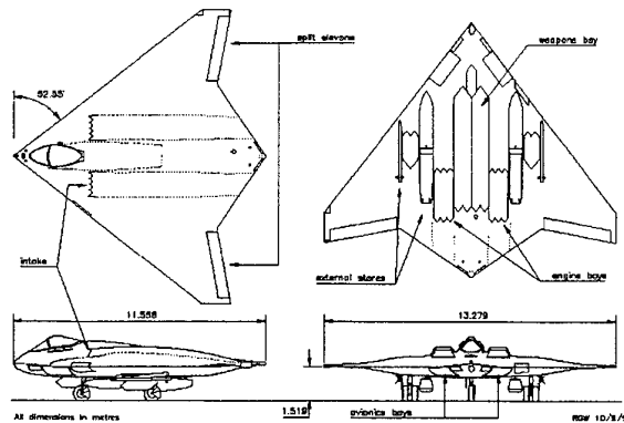
Figure 13. Final LSV-F Configuration.
