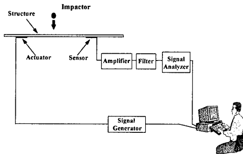
Fig. 1: The Acousto-Ultrasonics Principle
