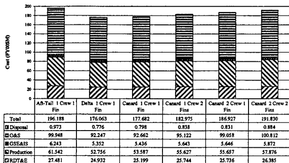
Figure 9. Twin-Engine LCC Breakdown.
