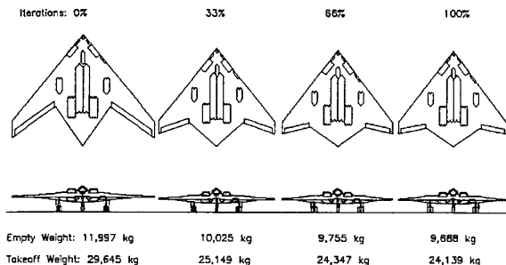
Figure 12. Optimiser Evolution of the LSV-F.
