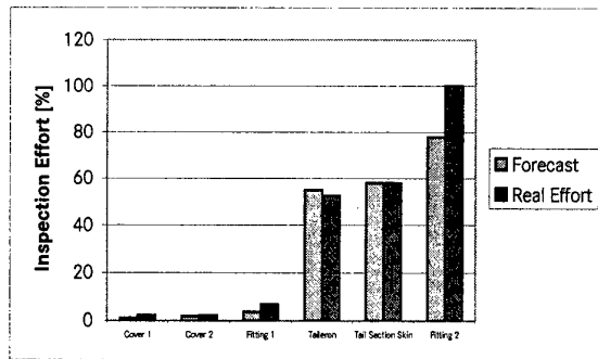
Fig. 14: Validation of the CER Model
