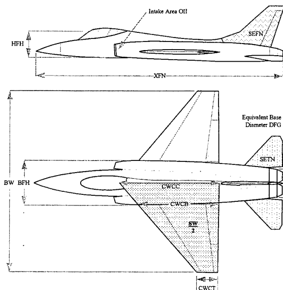
Figure 2. Aircraft Variable Definitions.
