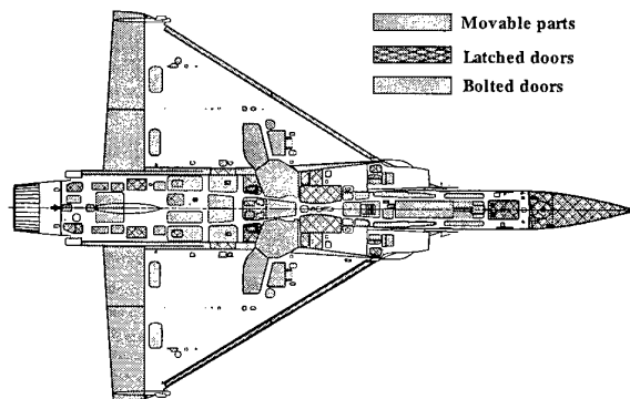
Figure 2 : MIRAGE 2000 access doors.
