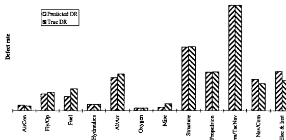
Figure 16. Predicted and Recorded Defect Rates, By System.
