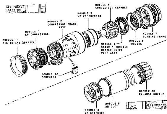
Figure 3 : Exploded view of SNECMA M53 engine
