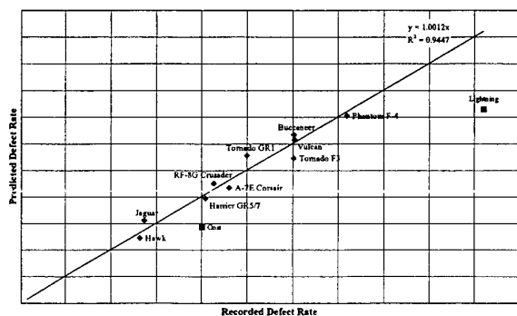
Figure 15. Predicted vs. Recorded Defect Rates.
