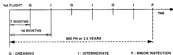
Figure 5 : Basic and minor inspections
