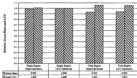
Figure 11. Relative Mass & LCC - Mass vs. LCC-Optimised.
