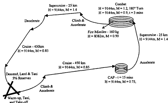
Figure 6. Aircraft Mission Performance Requirements.
