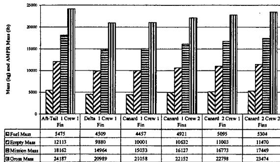
Figure 8. Twin-Engine Mass Breakdown.
