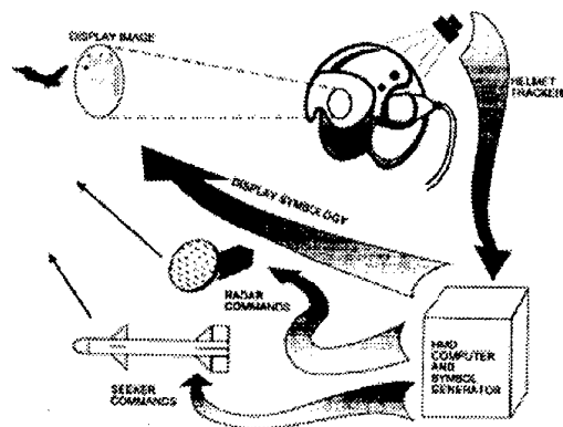
Figure 6.1. Schematic of Helmet Mounted Display/Tracker System Concept.
