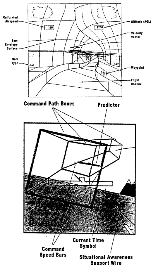
Figure 6.5. Examples of Pictorial Pathway-in-the-Sky Flight Display Formats [22,23].
