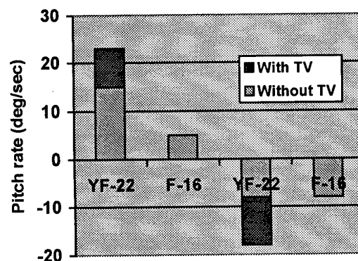
Figure 4 : Maximum pitch up, pitch down of the YF22 aircraft [6].
