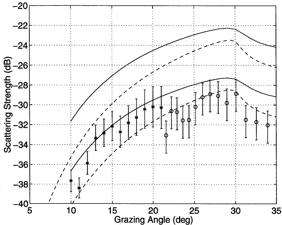
Figure 2. Bottom backscattering strengths at 40 kHz. The circles and asterisks denote results from STMS and BAMS, respectively. The two sets of curves are the uncertainty bounds for model results based on fluid (solid curves) and Biot (dashed curves) models for the sediment using roughness data measured near BAMS.
