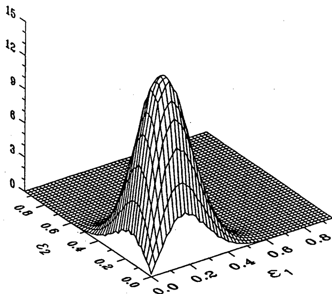
Figure 4. Comparison of the analytic FHO-FR probability and the numerical DIDIAV probability of the V-T transition (1,0 \rightarrow 0,0) for \text{N}_2\text{-N}_2 , both averaged over the collision angles \vartheta_1, \vartheta_2, \varphi_1 , and \varphi_2 , as functions of the rotational energies \epsilon_1 and \epsilon_2 . The total collision energy is E=1000 \text{ cm}^{-1} , b=0 .
