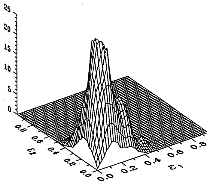
Figure 4. Comparison of the analytic FHO-FR probability and the numerical DIDIAV probability of the V-T transition (1,0 \rightarrow 0,0) for \text{N}_2\text{-N}_2 , both averaged over the collision angles \vartheta_1, \vartheta_2, \varphi_1 , and \varphi_2 , as functions of the rotational energies \epsilon_1 and \epsilon_2 . The total collision energy is E=1000 \text{ cm}^{-1} , b=0 .
