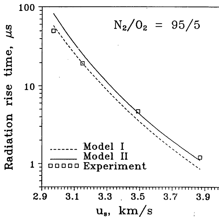
Figure 6. NO IR radiation rise time (time to the half-maximum) as a function of the shock velocity. \text{N}_2/\text{O}_2 = 95/5
