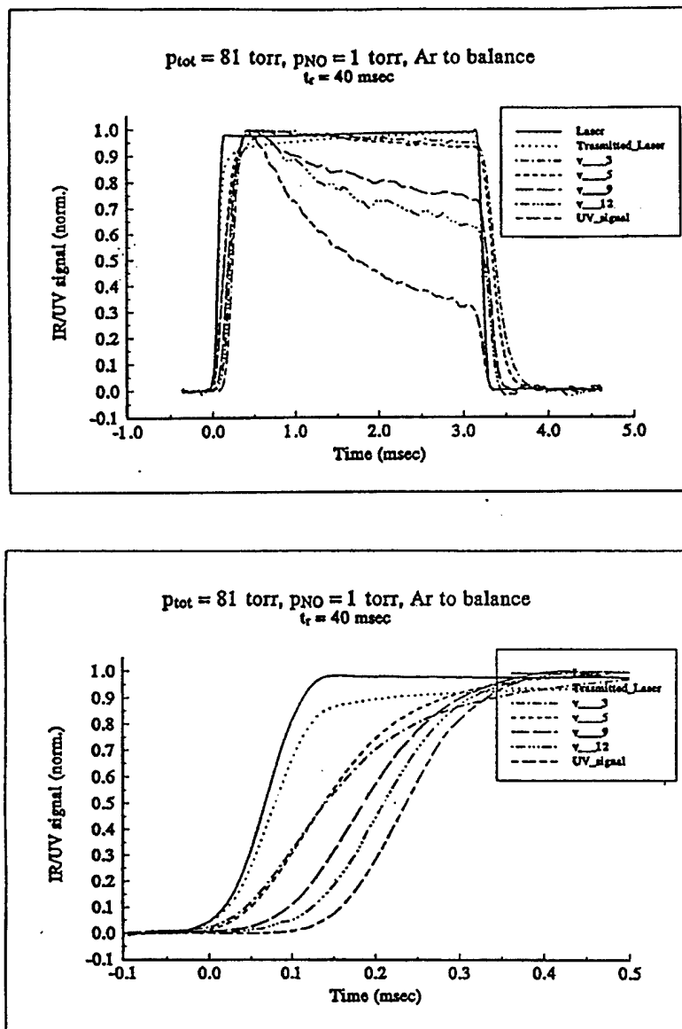
Figure 4. Time-dependent IR and UV emission from the optically pumped NO in the cell. P_{\text{NO}} = 1.0 torr
