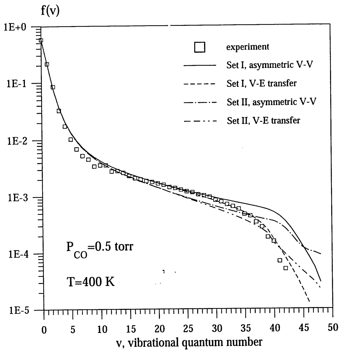
Figure 7. Experimental and theoretical steady-state CO distribution functions at P_{CO} = 0.5 \text{ torr}
