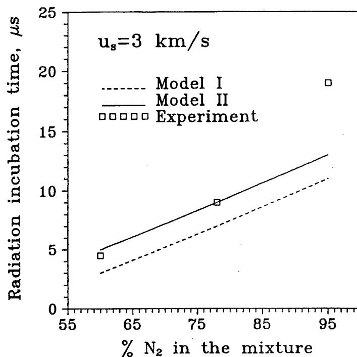
Figure 5. Experimental and calculated NO IR radiation incubation time at u_s = 3 \text{ km/s} as a function of the nitrogen mole fraction in the mixture
