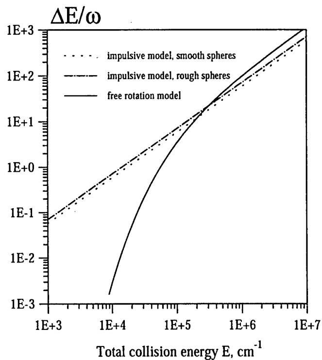
Fig.1a, b. Average number of quanta transferred to initially non-vibrating oxygen molecule versus total collision energy, as given by impulsive and free-rotation models. (a) \text{O}_2\text{-Ar} collisions; (b) \text{O}_2\text{-O}_2 collisions
