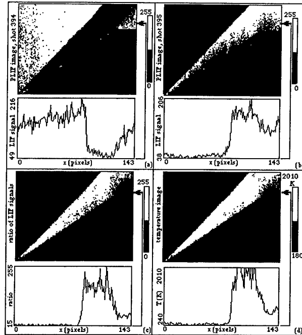
Figure 5. Images and profiles: (a) Fluorescence from excitation of the R 2 (15) line of NO; (b) fluorescence from excitation of the Q 1 +P 21 (25) line of NO; (c) ratio of fluorescence intensities from these respective images; (d) inferred temperature. The wedge angle is 35°, the distance from the base of the image to the shoulder of the wedge is 12.7 mm, and the profiles are taken along a horizontal line 8 pixels (1.3 mm) above the shoulder.
