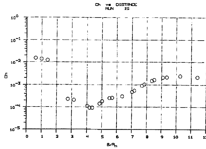
Figure 2-12a Distribution of Heat Transfer Coefficient over Planetary Probe Model and Sting for Case C Test Condition (Run 15)
