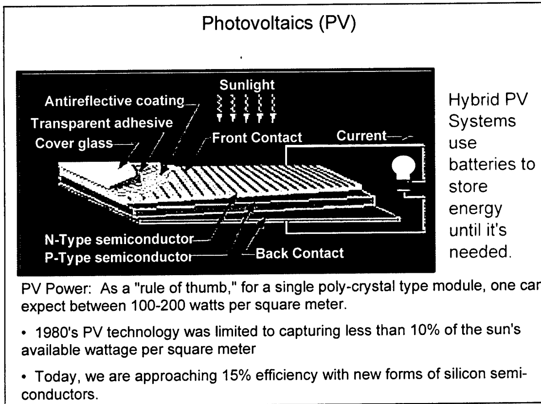
Figure 7. How PV Works
