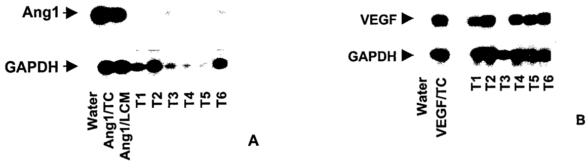
Figure 3. Expression of Ang1 and VEGF in tumour specimens determined by using laser-capture microdissection. (A) Detection of Ang1 expression in 6 tumour specimens, by RT-PCR and subsequent Southern analysis. Controls are RNA isolated from Ang1 transfected cells growing in culture (Ang1/TC) or microdissected from a section of a cell pellet (Ang1/LCM). (B) Detection of VEGF in the same cancer specimens by RT-PCR and Southern analysis.
