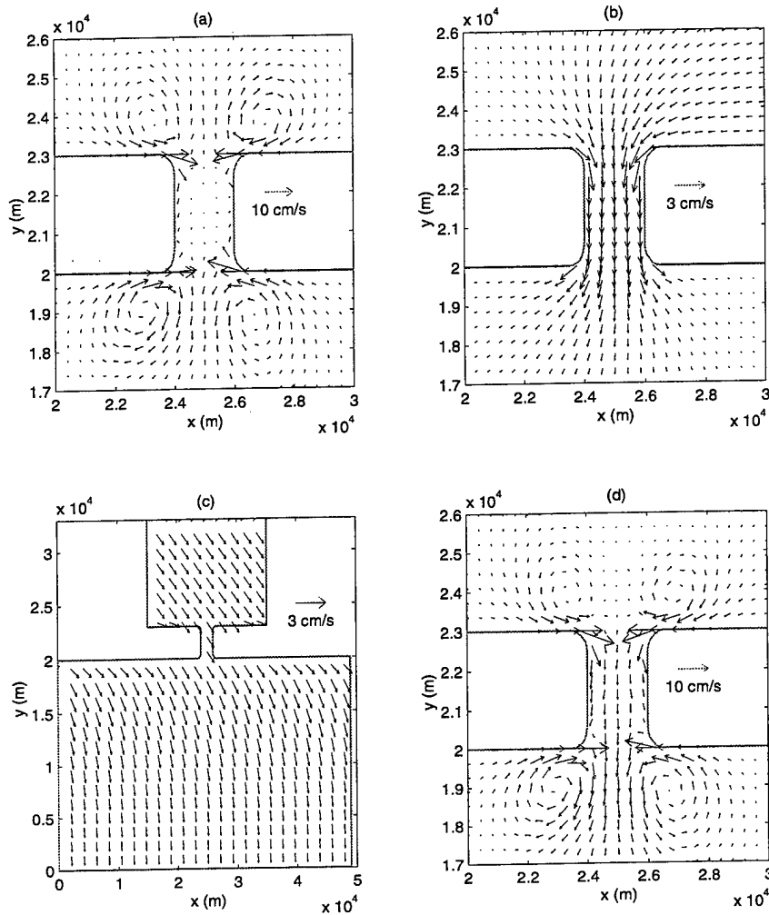
Fig. 8 – Residual velocities forced by (a) tide only; (b) river runoff only; (c) wind only; (d) combination of tide, river runoff, and wind.
