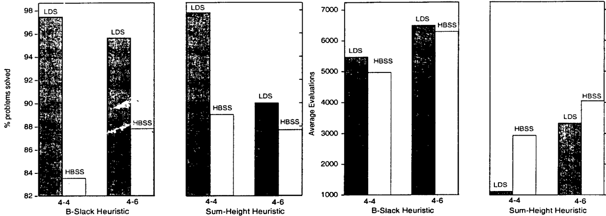
Figure 8: The two leftmost graphs show the percentage of feasible instances solved by B-Slack and Sum-Height, using LDS and HBSS. The two rightmost graphs show the average number of evaluations to solve feasible instance solved by B-Slack and Sum-Height, using LDS and HBSS.
