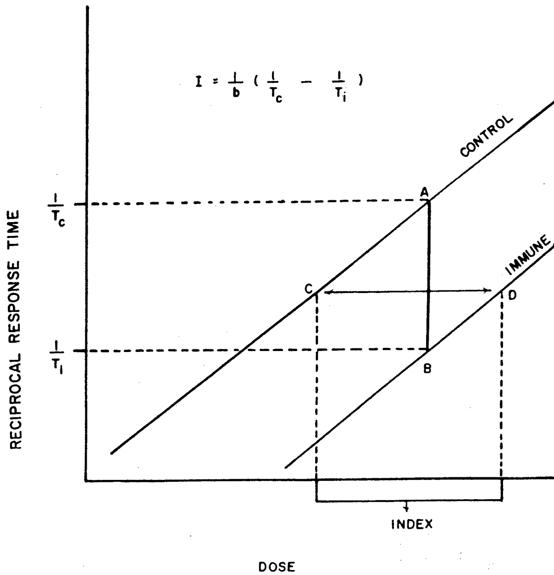
Figure 2. Immunity Index.
