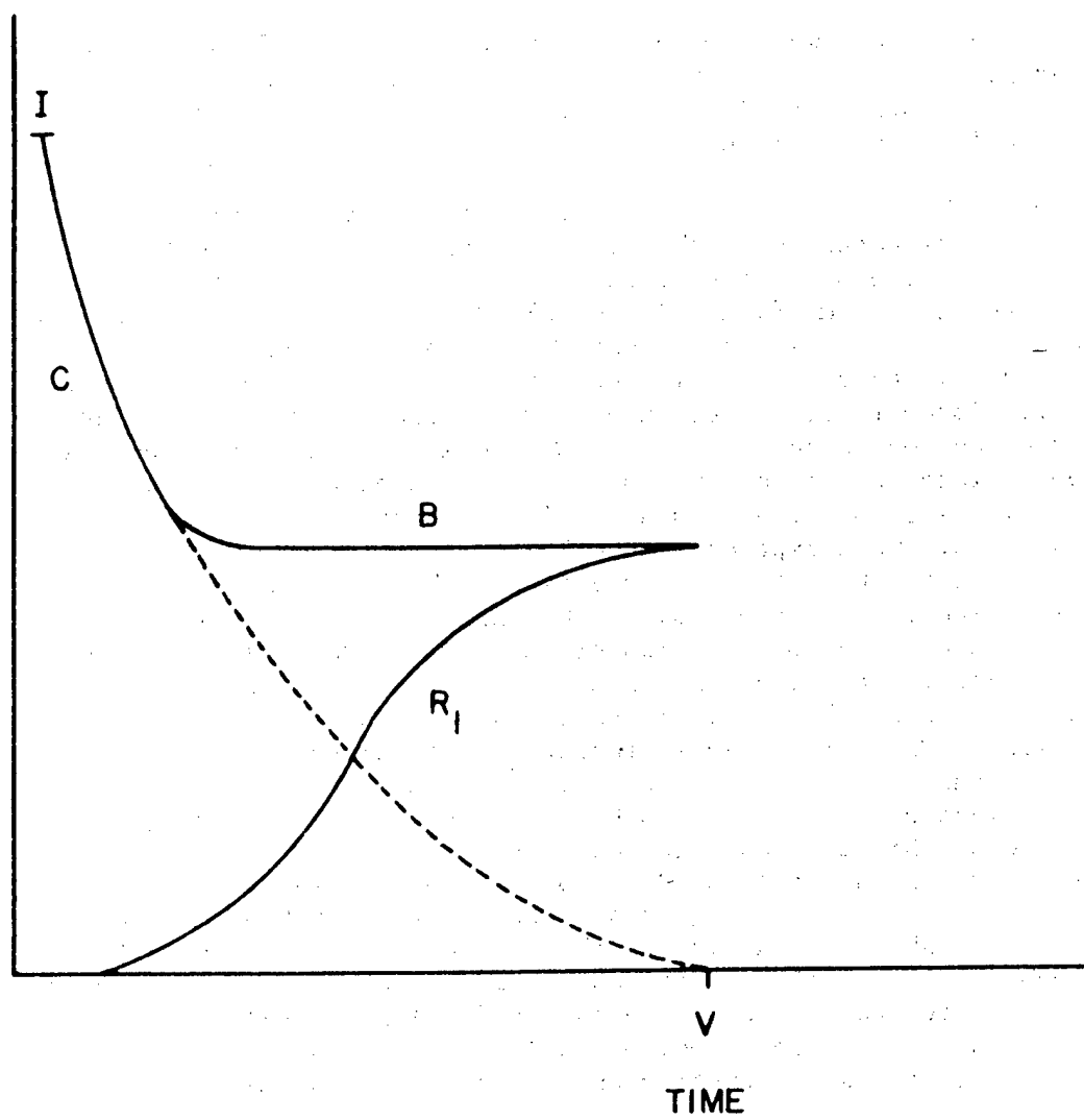
Figure 17. Anthrax Model 2.
