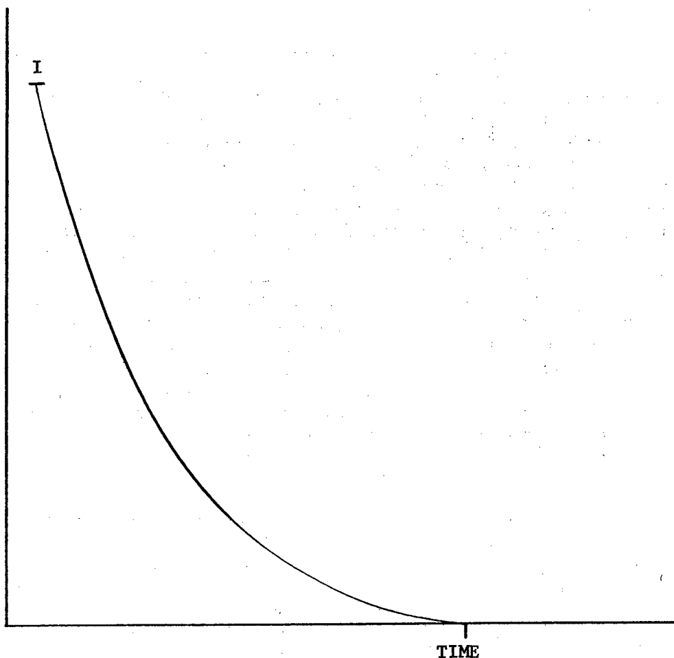
Figure 16. Anthrax Model 1.
