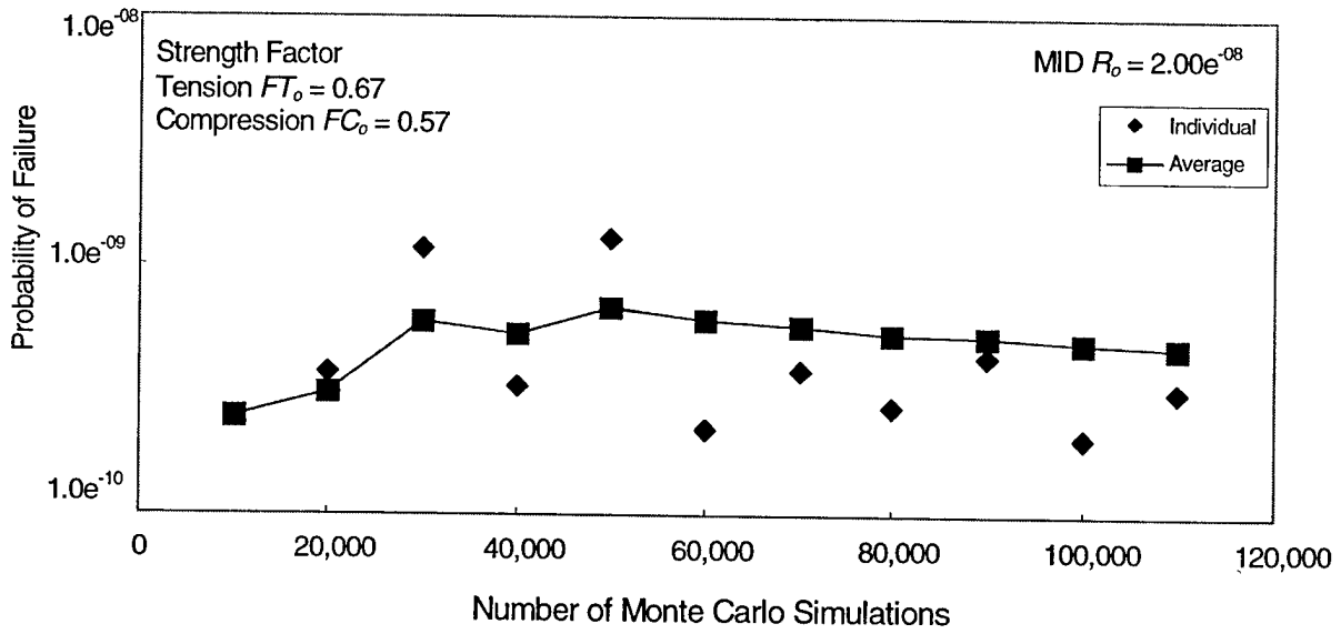
FIGURE 21: OVERALL P_f FOR R_0 = 2.00e^{-08}
