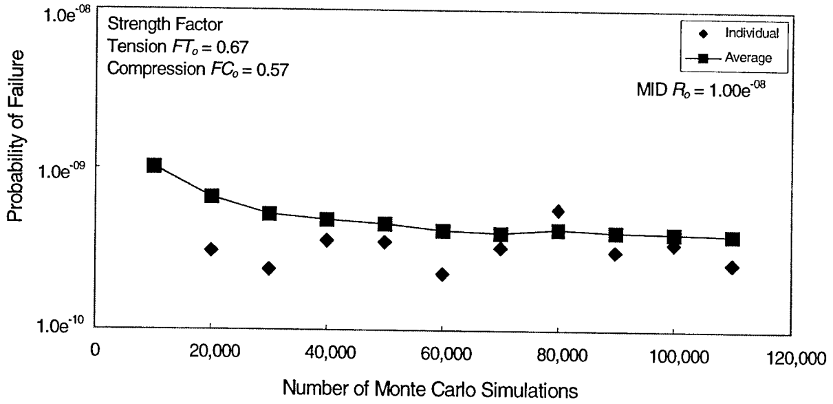
FIGURE 20. OVERALL P_f FOR R_0 = 1.00e^{-08}
