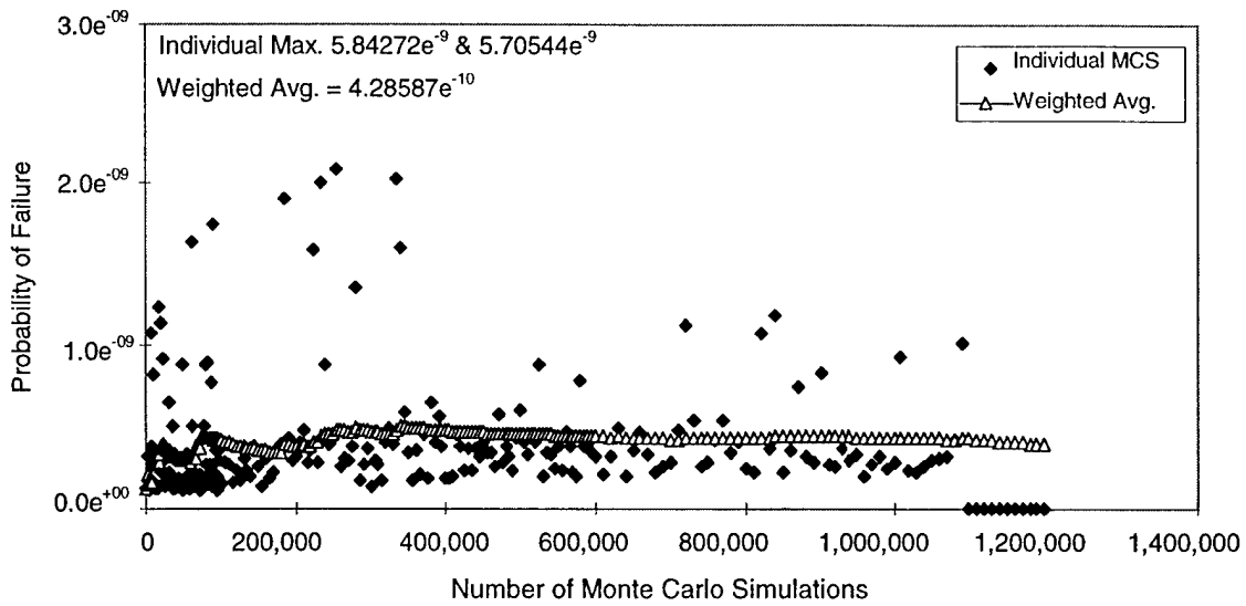
FIGURE 12. AVERAGE PROBABILITY OF FAILURE FOR THE OVERALL LEAR FAN MODEL, COMBINED RESULTS
