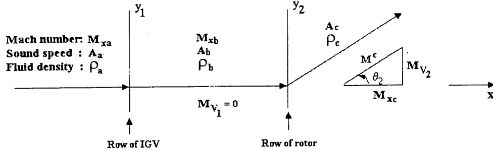
Figure 6.7: Schematic diagram of the 2D cascade model for the simulator.
