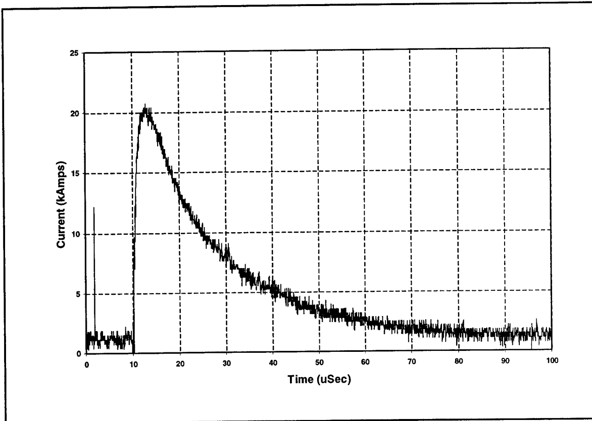
Figure 2. Typical Current Pulse
