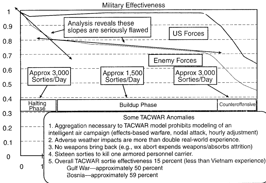
Figure 2. TACWAR Anomalies
