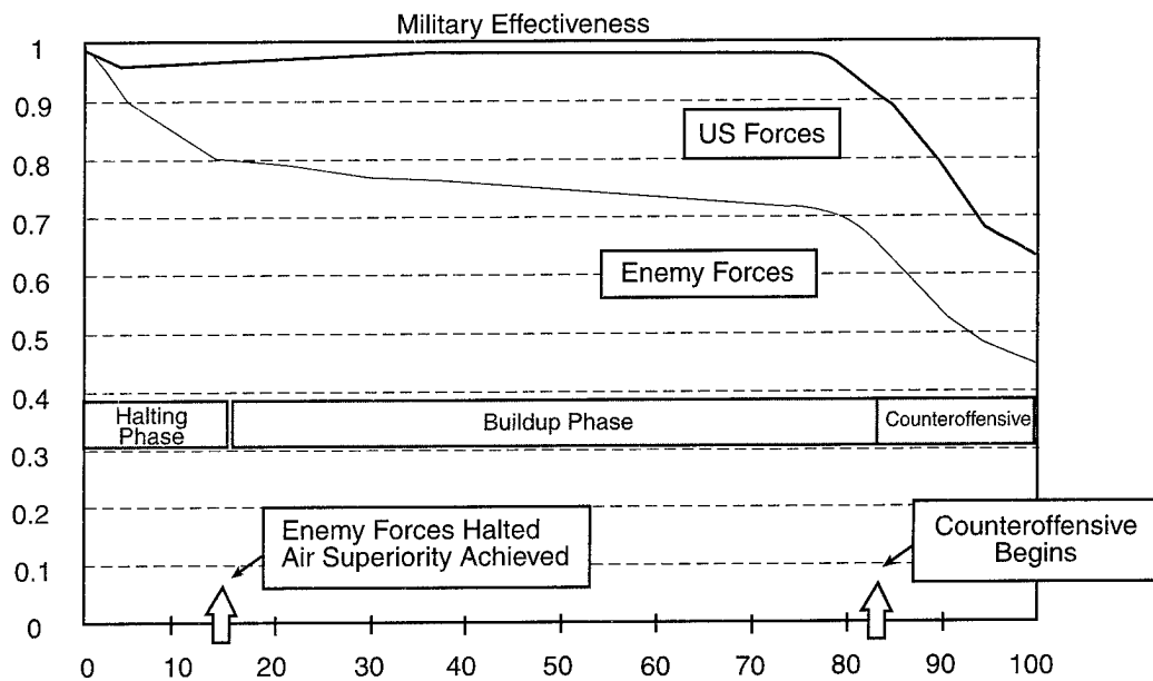
Figure 1. TACWAR Model
