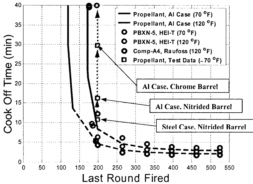
Figure 15. Prediction of propellant and explosive cook-off times for the 524 round magazine fire-out (combat tactical schedule).
