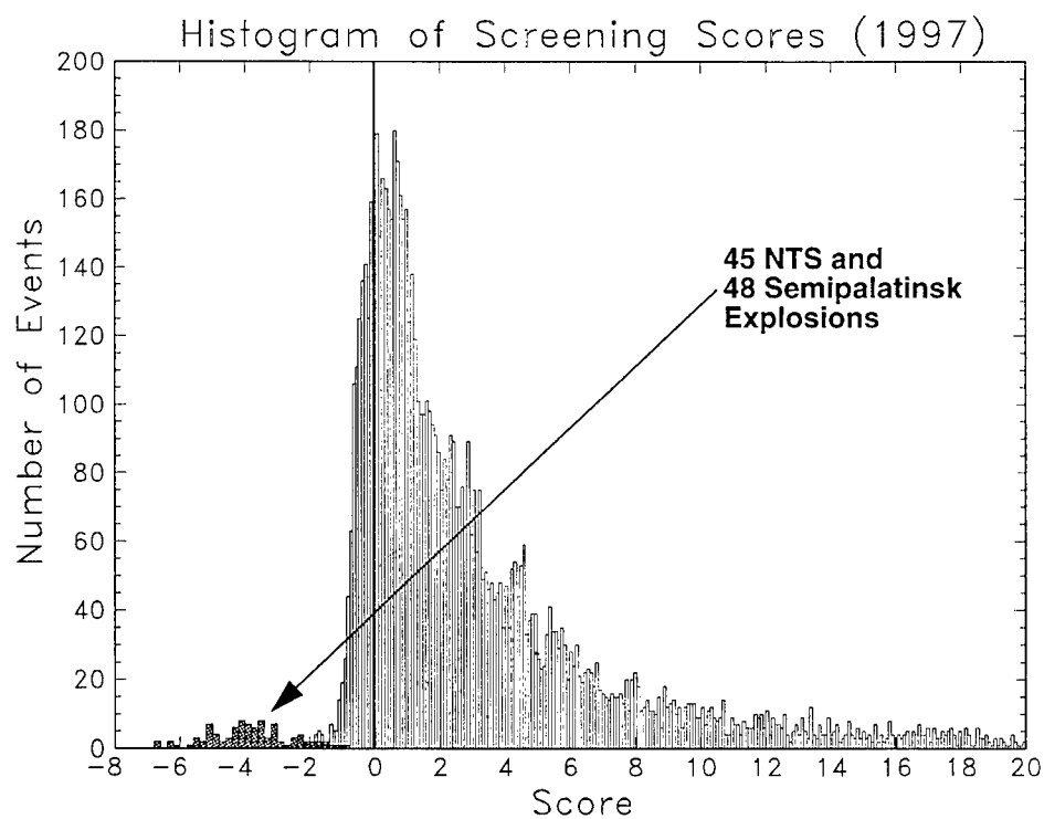
Figure 9. Histogram plots of the combined scores for all REB events with mb above 3.5 and M_s and/or unconstrained depth estimates during 1996 (upper plot) and 1997 (lower plot). The 96/06/08 Lop Nor explosion has the lowest score of all the events during these two years.
