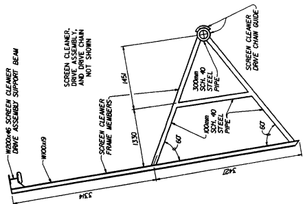
SCREEN CLEANER FRAME SIDE VIEW
