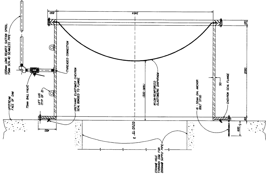
TEMPORARY BULKHEAD ASSEMBLY - SECTION
