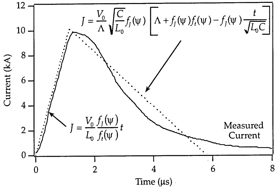
Figure 5.3: Variable element model for the current of a GFPPT discharge compared to a measured current trace from PT9: 4 J per pulse, 2.0 μg argon, 130 μF, 1" × 1" electrodes.
