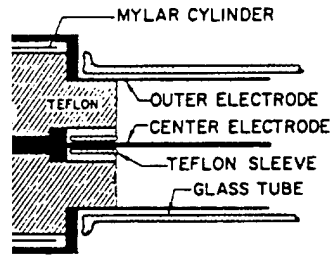
Figure 1.9: Schematic of Lockheed GFPPPT with large radius ratio and Teflon backplate. Taken from Ref. [29] and modified to remove extraneous information on distributed inductance and physical discharge switch.
