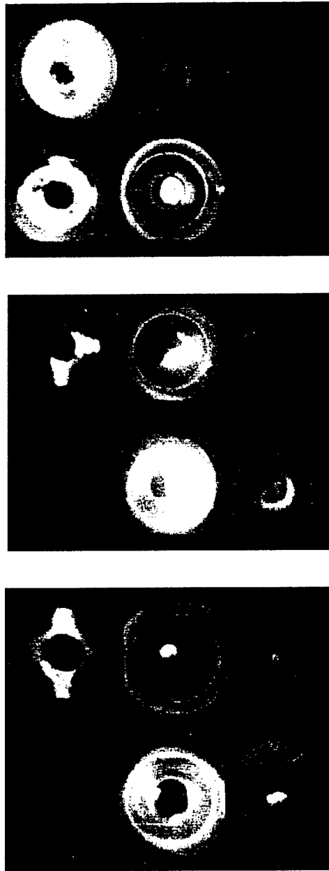
Figure 4.5: The 180 \mu\text{F} SRL4-GFPPT firing at 8 and 5 J/pulse with a 1.0 \mu\text{g} argon mass bit. The top picture shows an 8 J pulse, and the middle and bottom picture show a 5 J pulse. Framing rate: 2 \mu\text{s} per image with delays of 1.2 \mu\text{s} , -1.0 \mu\text{s} , and -1.1 \mu\text{s} for the top, middle, and bottom pictures, respectively. The delay on the middle and bottom pictures are negative because the first frame is taken before the discharge begins and is, therefore, blank.
