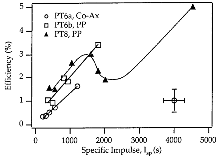
Figure 3.4: Efficiency vs. specific impulse for PT6 and PT8 with argon at various mass bits. All data shown is taken at 2 J per pulse using a 63 \mu\text{F} capacitor. A proportional error bar for the middle of this data set is also shown.
