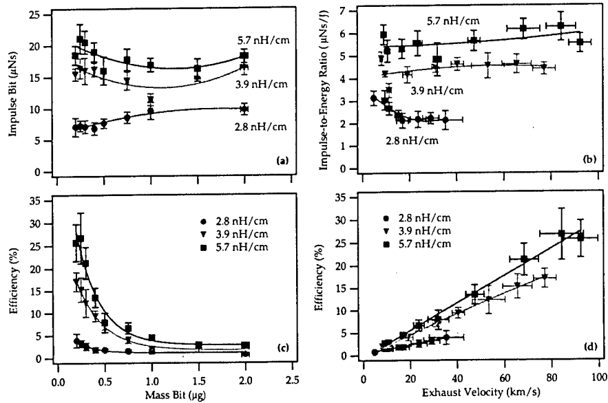
Figure 5.9: Measured performance of PT9 with argon, a 130 \mu\text{F} capacitor bank, approximately 4 \text{ J/pulse} and the inductance-per-unit-length as a parameter. Graphs (a) and (c) show the impulse bit and thruster efficiency as a function of mass bit. Graphs (b) and (d) show the impulse-to-energy and thruster efficiency as a function of exhaust velocity.
