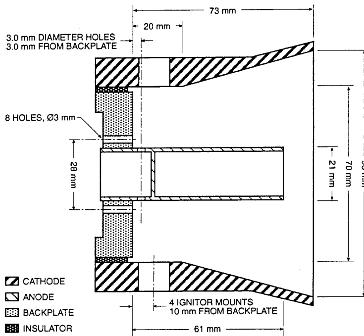
Figure 1.16: Schematic of SRL-EPPDyL PT5.
