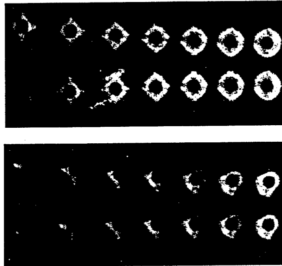
Figure 4.4: The 270 \mu\text{F} SRL4-GFPPT firing at 5 J/pulse with a 0.5 \mu\text{g} argon mass bit. Framing rate: 50 ns per image with a 0.8 \mu\text{s} delay on both.
