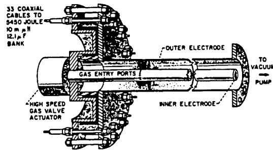
Figure 1.11: Schematic of NASA Lewis "Gun A" GFPPPT. Taken from Ref. [35].
