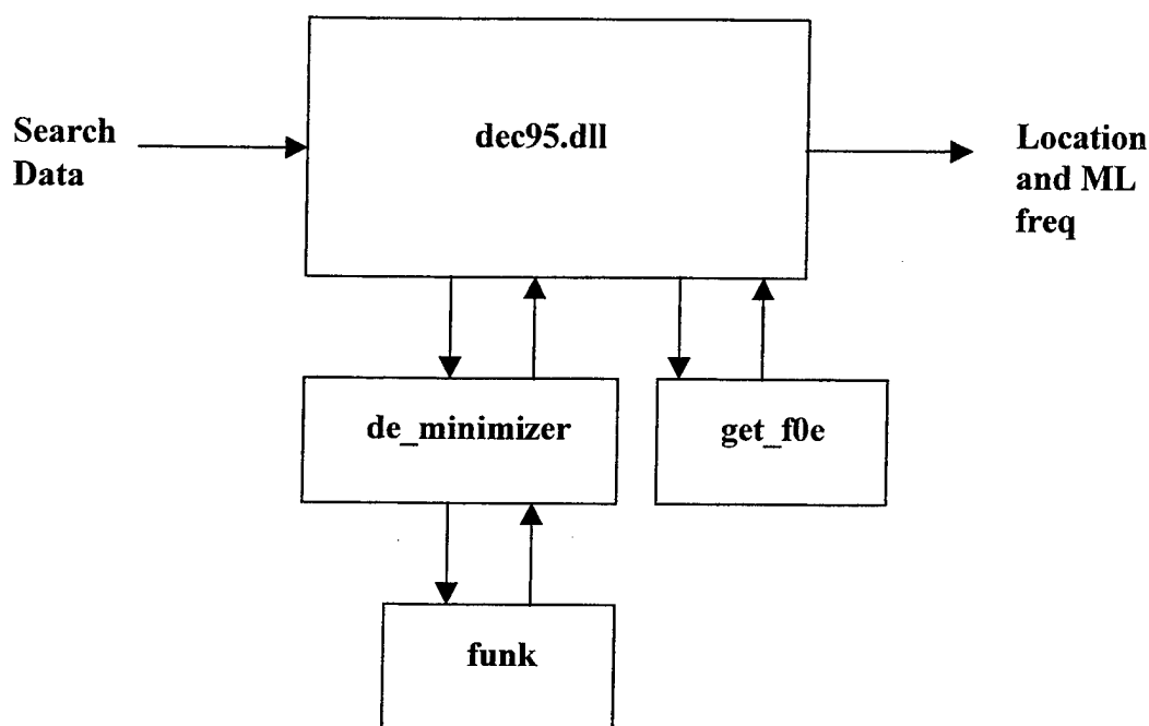
Figure 9: Overview of the Differential Evolution DLL
