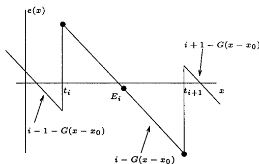
Figure 2: Static Error Description
