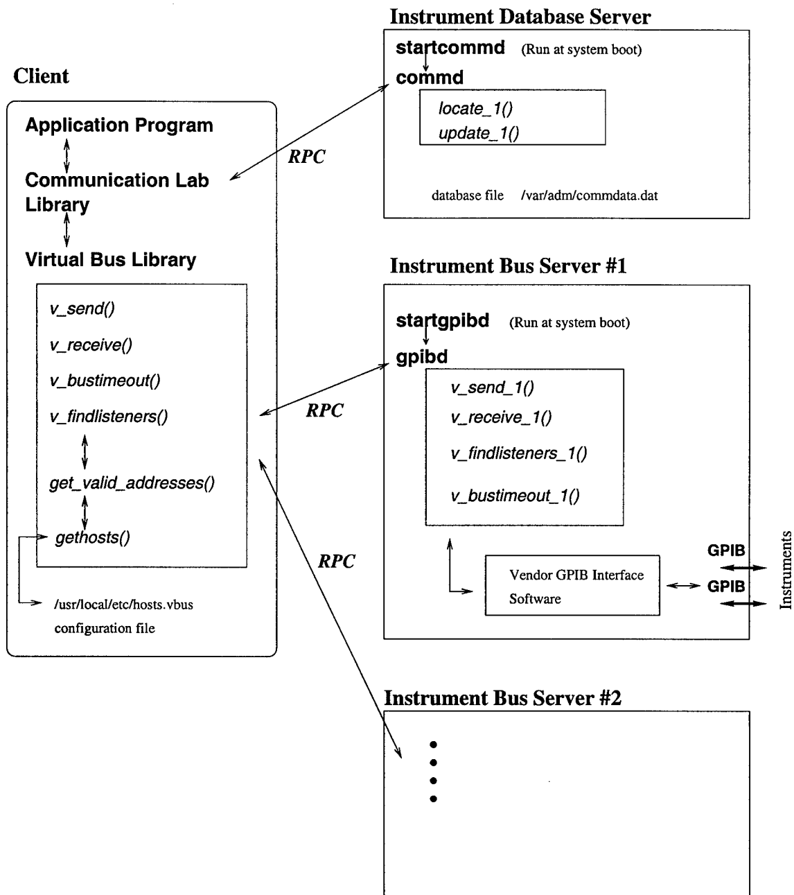
Figure 4: Software Architecture
