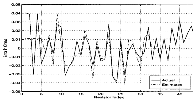
Figure 4. Actual vs Estimated Errors in CDP Reference Resistors
