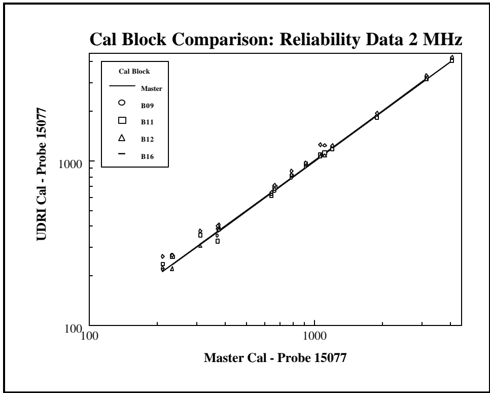
Figure 33 - Comparison of 2 MHz reliability results using probe 15077.
