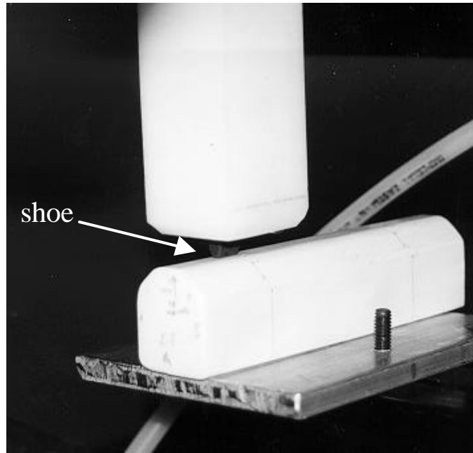
Figure 40 - An eddy current probe shoe was used to conduct wear tests on the wire-artifact calibration blocks.
