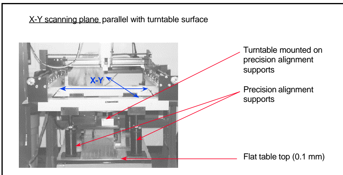
Figure 1 - Mechanical frame, motorized axes, and alignment fixtures of the eddy current data acquisition system used to develop the new calibration blocks.
