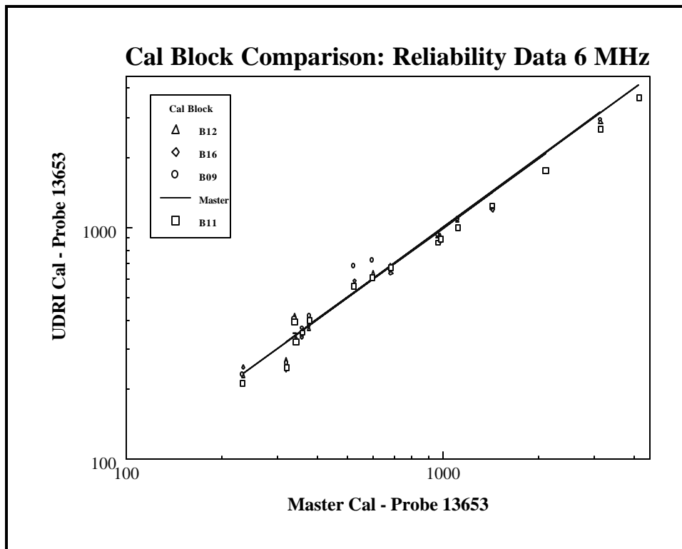
Figure 32 - Comparison of 6 MHz reliability results using probe 13653.
