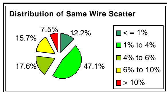
Figure 21 - The uniformity of eddy current response along any given wire is shown by a pie chart of the variations from an average response.
