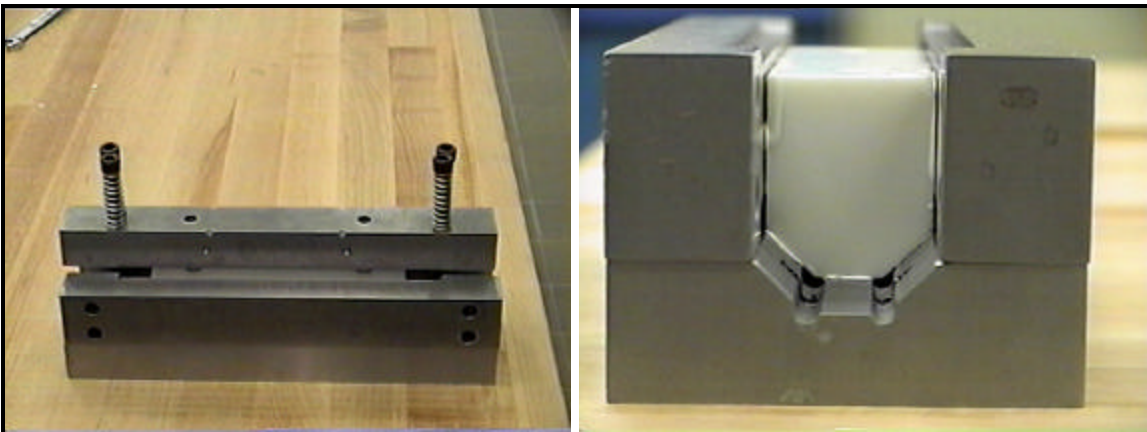
Figure 16 - A mold was created to allow simultaneous construction of all five sides of the wire-artifact blocks.
