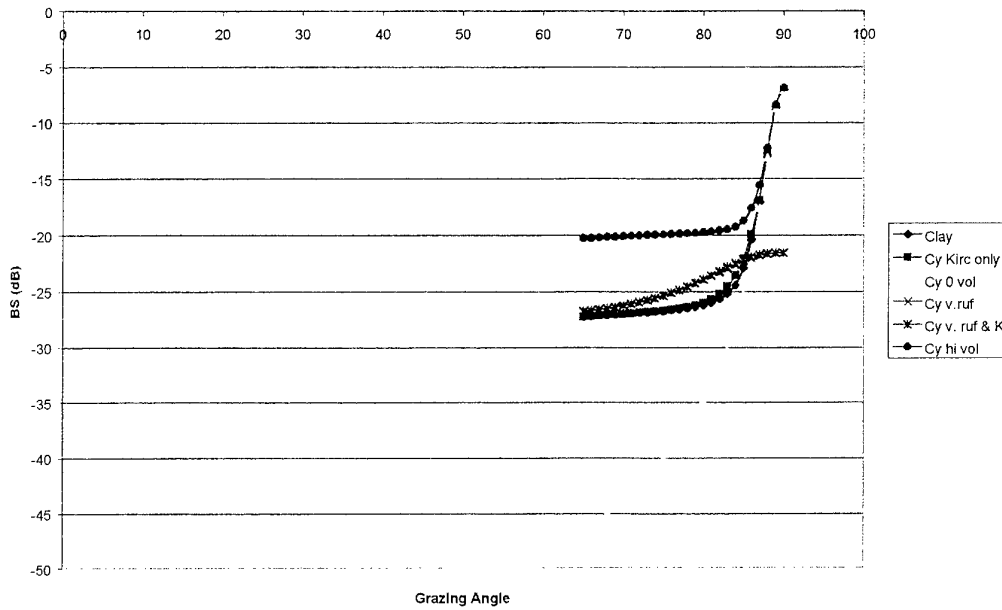
Figure 5. Backscatter versus grazing angle curves for clay.
