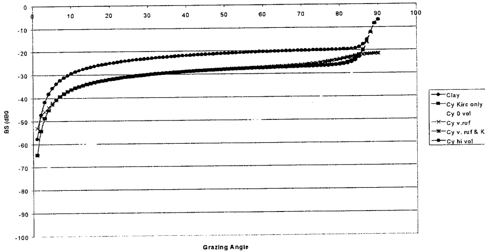
Figure B2. Backscatter versus grazing angle curves for clay.
