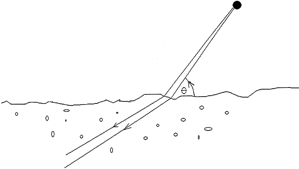
Figure 1. Sketch of geometry for backscatter versus grazing angle models.
