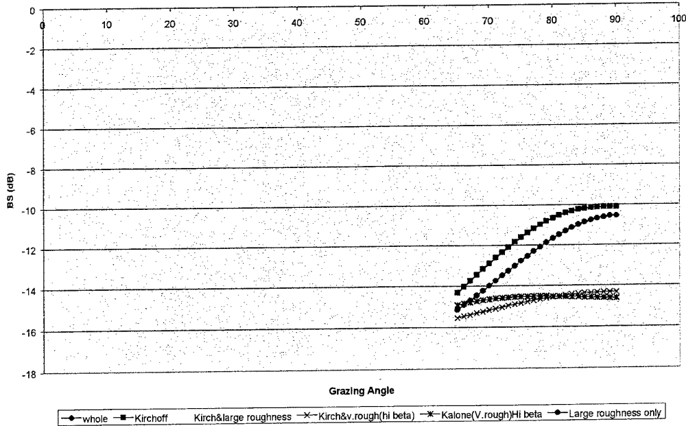
Figure 10. Backscatter versus grazing angle curves for very coarse sand.
