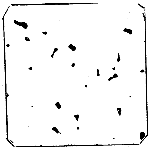
Scale of a microstructure with residual microporosity (six levels) b (x100)
