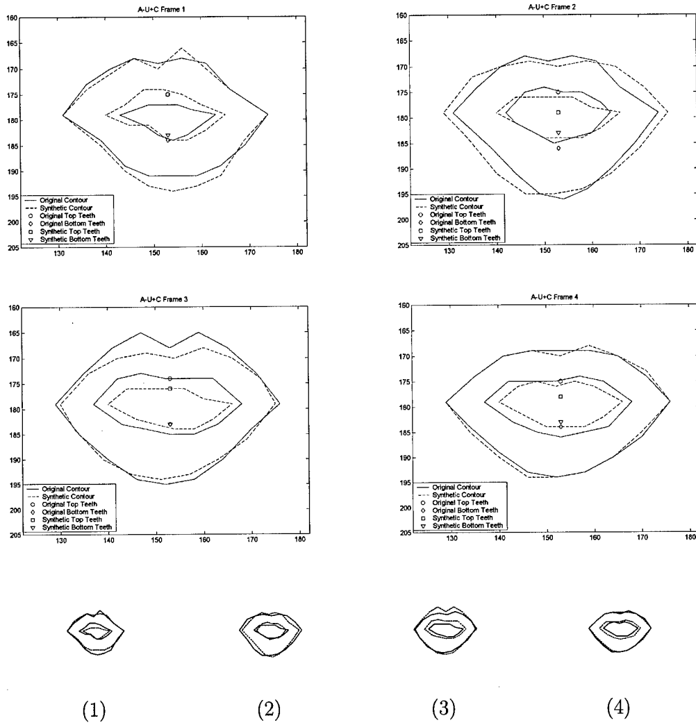
Figure 35. A-U+C T = 20, R = 20, \Theta = 1 , No Skip HMM.
