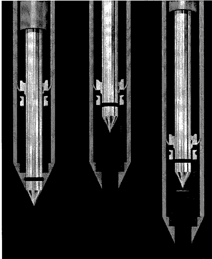
Figure 3. TDS probe sampler collection
