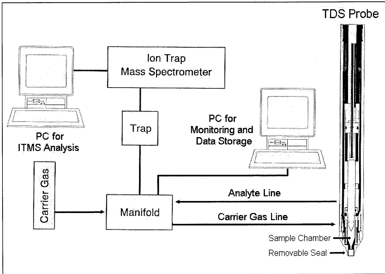
Figure 1. Thermal desorption sampler system
