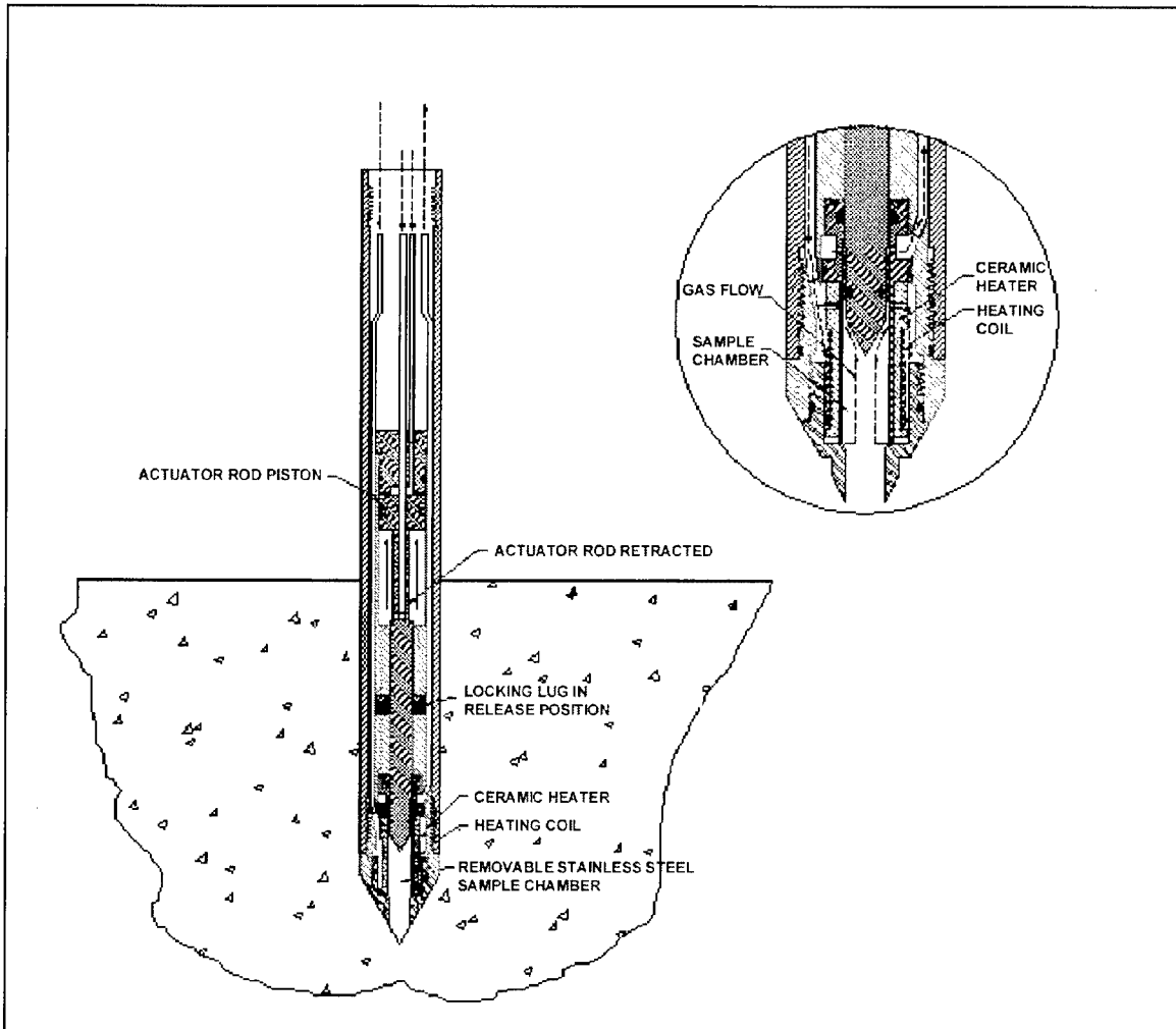
Figure 2. Thermal desorption sampler probe
