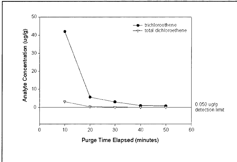
Figure 13. TDS system recovery after analysis of a highly contaminated sample
