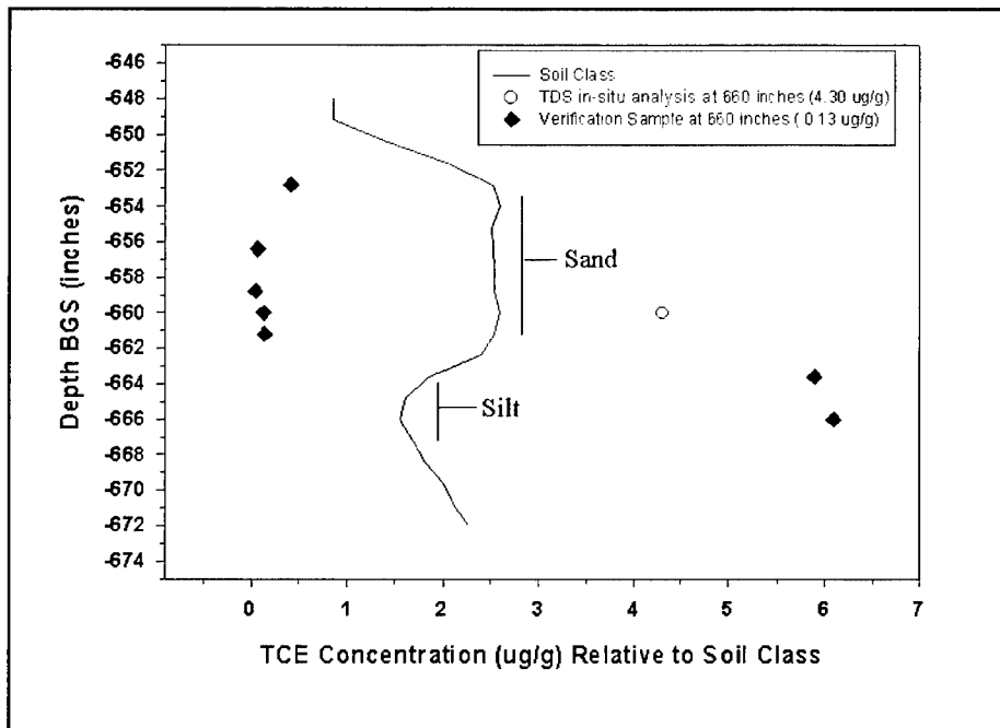
Figure 10. Changes in TCE concentrations at CRREL relative to soil type and depth. Soil class changes from sand to silt between 664 and 670 in. BGS
