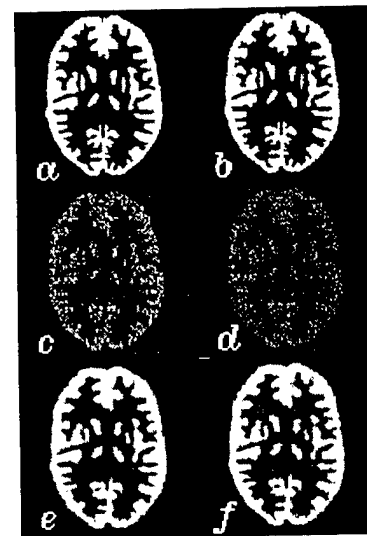
Figure 1. Reconstructions of a Hoffman brain phantom from simulated projections without noise (a-b) and with Poisson noise added (c-f). Reconstruction methods are: (a) FBP with ramp filter (cutoff=1.0), (b) direct-spline inversion using interpolating splines, (c) FBP with ramp filter (cutoff=1.0), (d) direct-spline inversion using interpolating splines, (e) FBP from a sinogram generated by sampling smoothing splines, (f) direct-spline inversion using smoothing splines.
