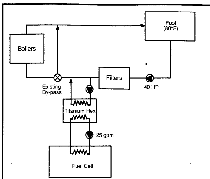
Figure 4. Fuel cell thermal interface—Port Hueneme.
