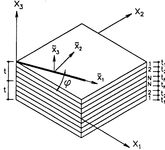
Figure 13 Geometry of a symmetric fibrous laminate.
