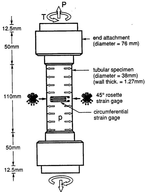
Figure 5 Dimensions and instrumentation of the composite tube specimen.
