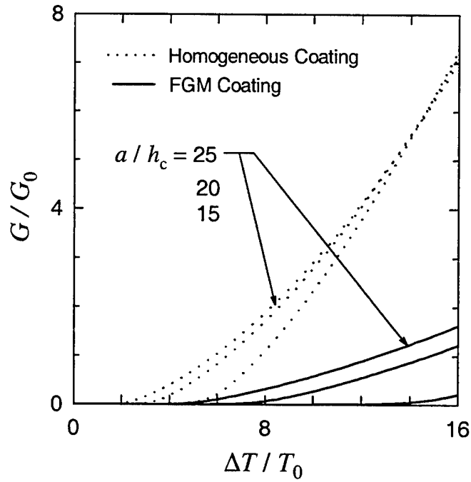
Figure 5.32 Strain energy release rate for homogeneous and FGM coatings under uniform temperature drop, T_0 = 100 K, K_0 = E_s \alpha_s T_0 \sqrt{\pi h_c} , G_0 = (1 - \nu_s^2) K_0^2 / E_s .
