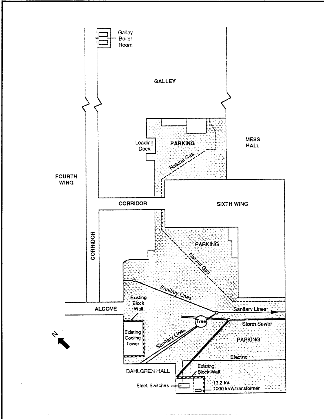
Figure 1. U.S. Naval Academy Dormitory/Gallery site layout.
