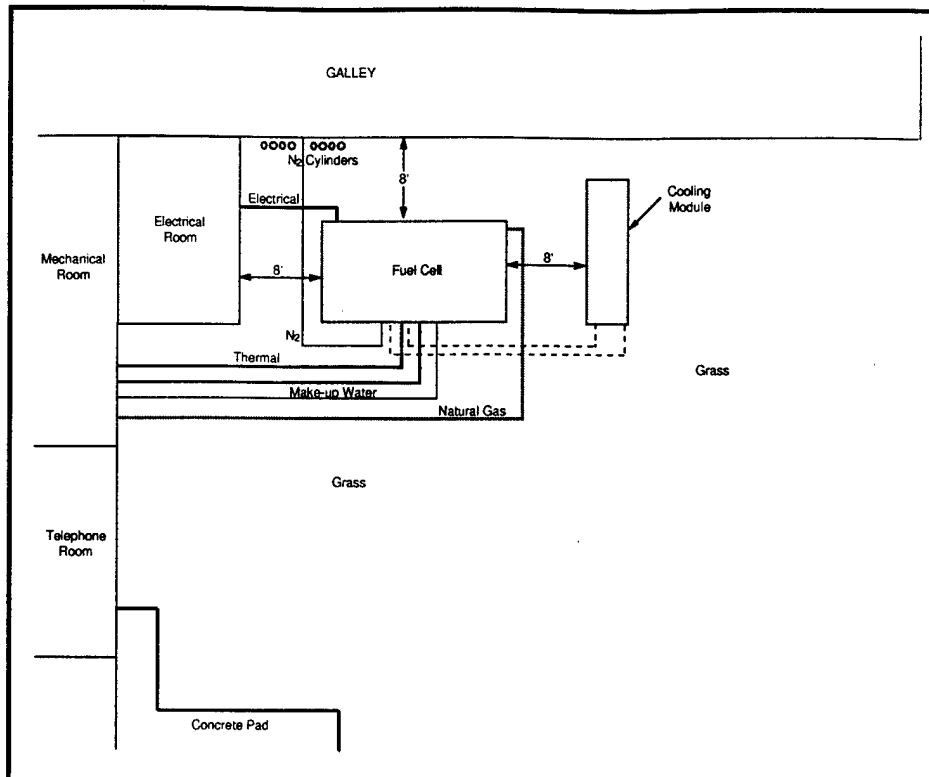
Figure 5. Fuel cell site layout — galley.
