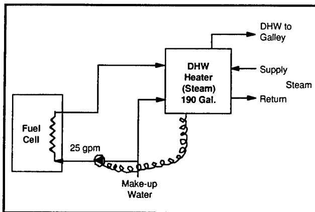
Figure 7. Fuel cell thermal interface — galley.
