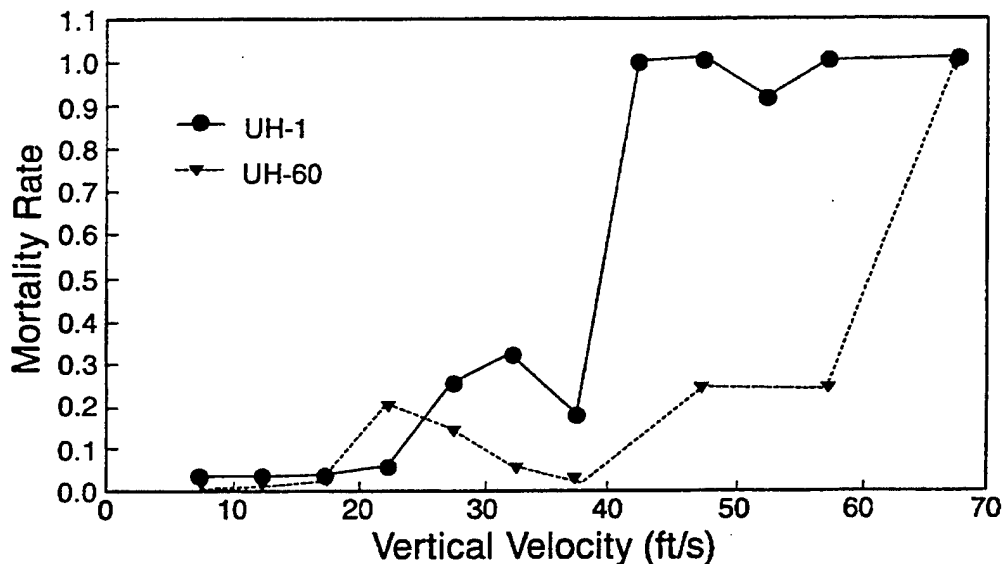
Figure 2. Mortality rate versus impact vertical velocity for UH-1 and UH-60.
