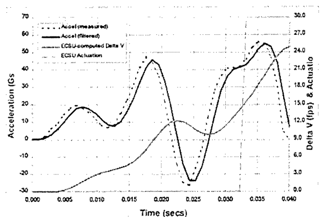
Figure 1. Example CABS ECSU Algorithm Operation: Actual CH-47 Crash Test Data.
