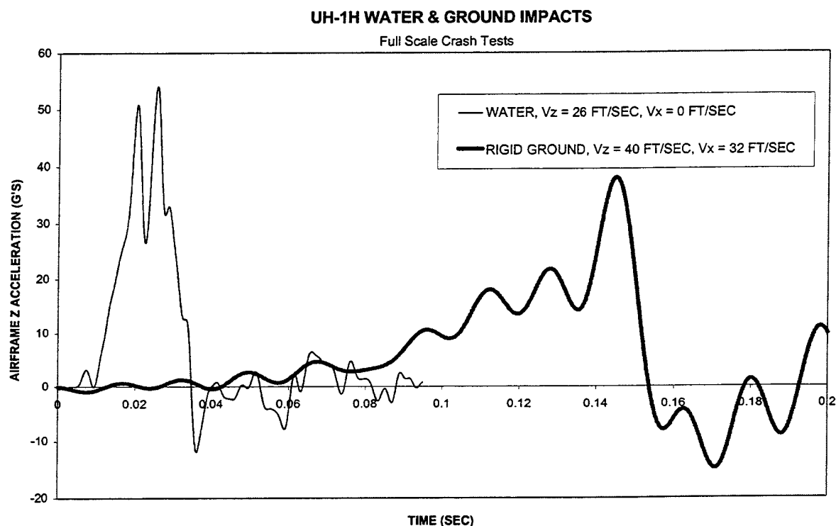
Figure 2: UH-1H Water and Ground Impact Results
