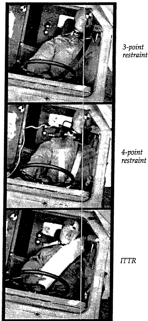
Figure 9. Rollover simulation in a military heavy truck.
