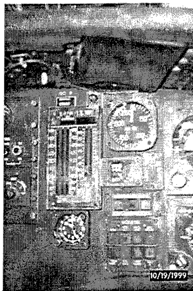
Figure 2 – Installation of Forward Air Bag Module in UH-60A
