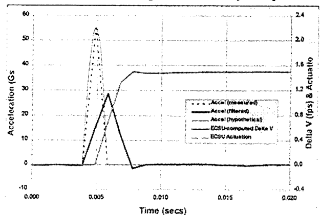
Figure 3. Hypothetical Case #1a: A 55-G, 2-msec Hammer Strike.
