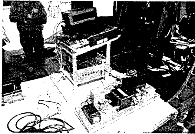
Figure 4 – Instrumentation Pallet
