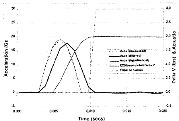
Figure 8. Hypothetical Case #1e: A 19-G, 5.9-msec Half-Sine-Wave Acceleration Pulse.
