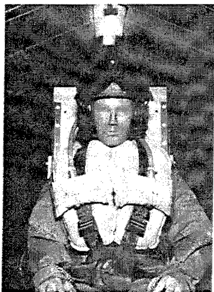
Fig.3 IBAHRS CDR system deployed
