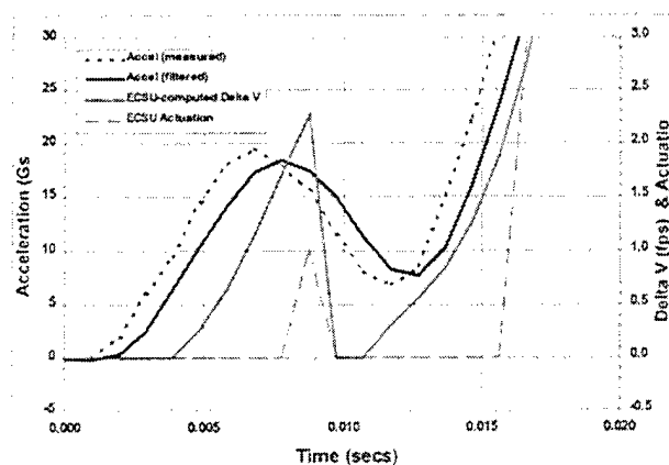
Figure 11. Hypothetical Case #2c: Actual CH-47 Crash Test Data.
