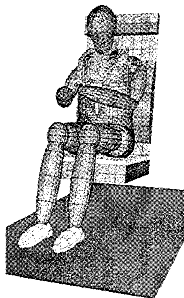
Fig.4 Typical computer model output of 10Gx impact
