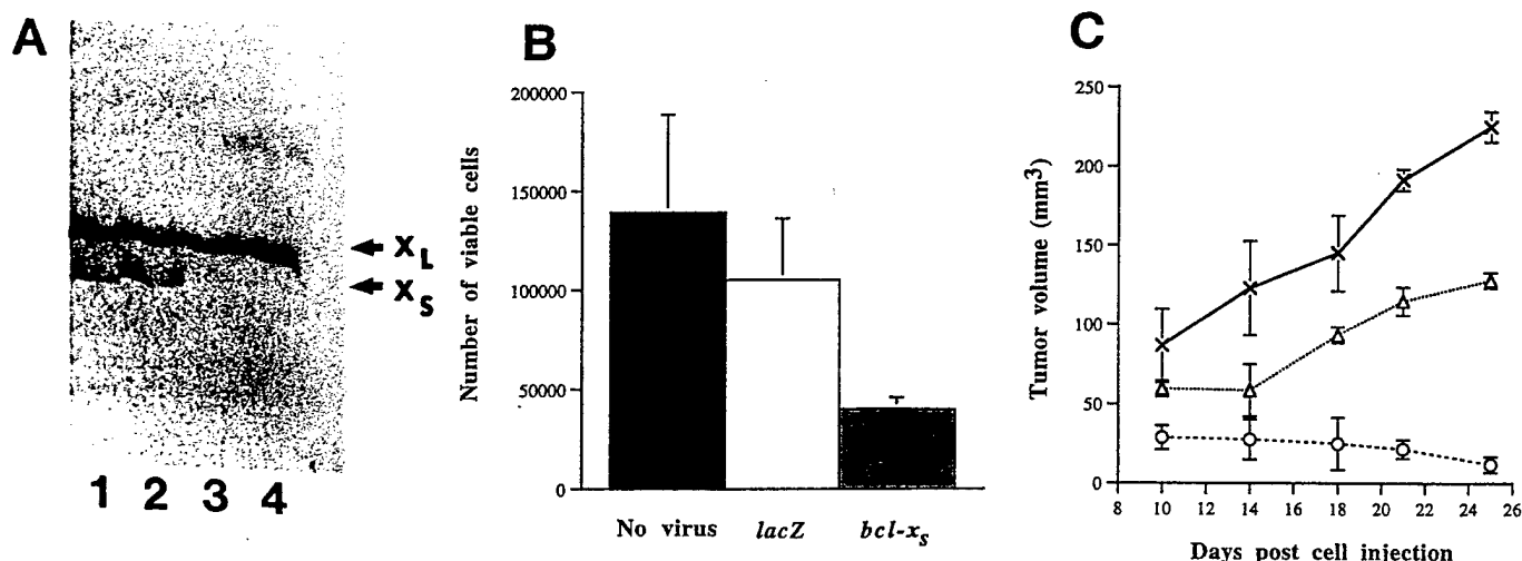
Fig. 1. Effects of Bcl- x s expression on cell viability. A, Western blot of Bcl- x expression. MCF-7 cells were infected as described in "Materials and Methods" with 2 \times 10^3 pfu/cell bcl-x s or lacZ adenovirus, and total protein lysates (400 \mu g/lane) were analyzed by Western blotting using a rabbit polyclonal antibody to Bcl- x . Lanes 1 and 2, bcl-x s -infected cells; lanes 3 and 4, lacZ -infected cells. Arrows: x L , Bcl- x L ( M r 25,630); x s , Bcl- x s ( M r 18,700). B, effect of bcl-x s adenoviral infection on MCF-7 viability. MCF-7 cells were infected in vitro with 10^4 pfu/cell bcl-x s or lacZ adenovirus. The number of live cells, as determined by trypan blue exclusion, was counted 5 days later ( P = 0.010; bars, SE; n = 3). C, effect of bcl-x s adenoviral infection on clonogenicity of MCF-7 cells. MCF-7 cells ( 3 \times 10^6 ) were treated with 10 pfu/cell bcl-x s or lacZ adenovirus in vitro and injected s.c. into opposite flanks of an estrogen-supplemented nude mouse. Tumor volume was calculated as described in "Materials and Methods" ( P = 0.0085; bars, SD; n = 2). \times , no virus; \Delta , lacZ ; \circ , bcl-x s .
