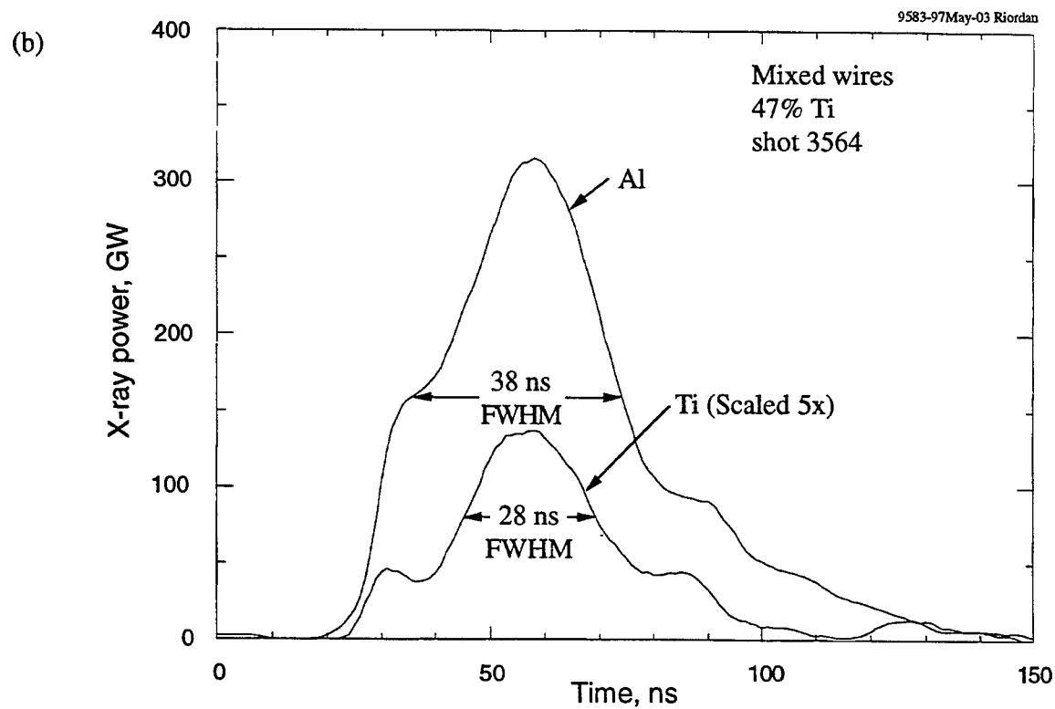
Figure 4-3. X-ray power in the aluminum and titanium spectral ranges for (a) coated wires with 48% Ti and (b) mixed wires with 47% Ti.
