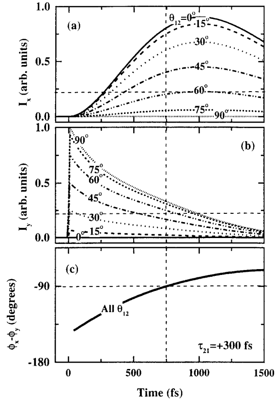
FIGURE 9.17. (a) The x component I_x(t) and (b) the y component I_y(t) of the TR-FWM intensity and (c) the phase difference, \phi_x(t) - \phi_y(t) , for selected angles \theta_{12} between the two input polarizations as calculated from the 2 \times 2 model modified to include EID, LFC, and BIF (i.e., calculated from the density matrix equations for the two-particle 5-level energy diagram of Figure 9.16 with EID and LFC included; see (9.20)). The time delay was fixed at \tau_{21} = +300 fs.
