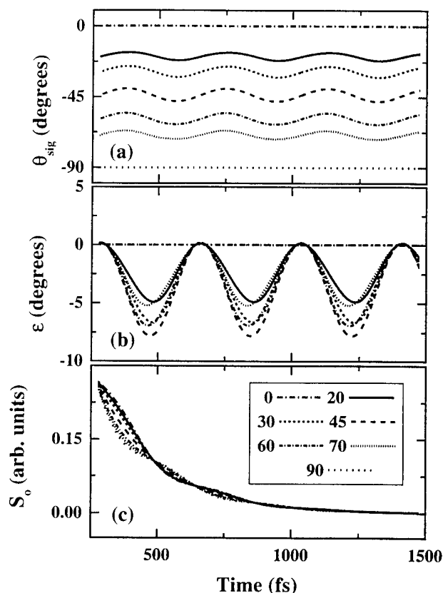
FIGURE 9.32. The two-independent-three-level-system ( 2 \times 3 ) simulations (without many-body effects) of the (a) azimuthal angle \theta_{\text{sig}} , (b) ellipticity angle \varepsilon , and (c) total intensity S_0 in the weak quantum beat regime for comparison with Figure 9.31.
