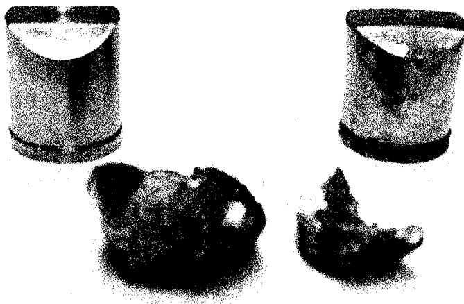
Figure 51: (left) 12.7 mm FSP(unfired), (right) 12.7 mm FSP recovered from shot 5 into target 1, (center foreground) aluminum shear plug from shot 5 into target 1, found almost completely detached from aluminum plate.
