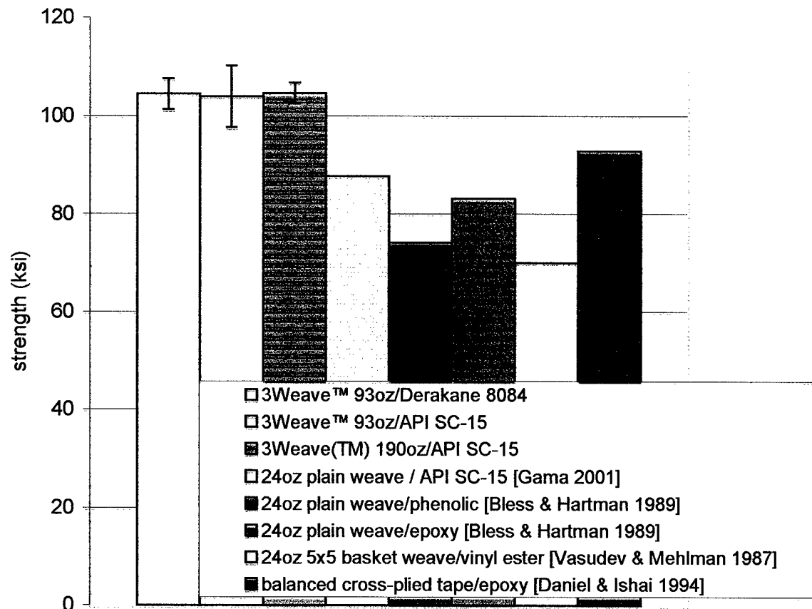
Figure 6: Warp tensile strengths of 3Weave™ S-2 Glass composites, compared to other S-2 glass composites considered for armor applications from the literature. Typical strengths of cross-ply laminates are also shown for comparison. Error bars on 3Weave™ values are standard deviations.
