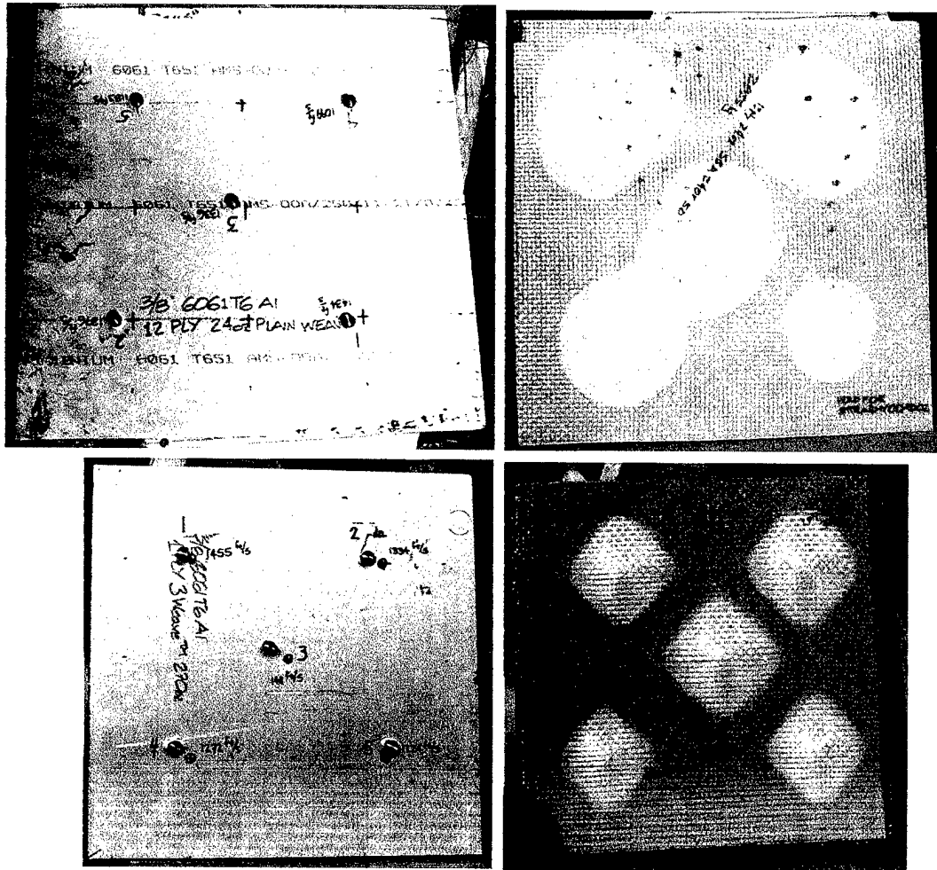
Figure 52: Targets after testing in non-perforating ballistic impact testing, consisting of 0.375-in 6061-T65 aluminum strike face (left), bonded to ~0.28-in S-2 glass composite backing plate (right). 18-in x 18-in target with 12 plies of 24-oz plain weave (the baseline fabric) in backing is shown at top. 16-in x 15.5-in target with one ply of 270-oz 3Weave™ (fabric 4) in backing is shown at bottom. Each target was shot five times with 12.7 mm FSP (shown embedded into the aluminum strike face).
