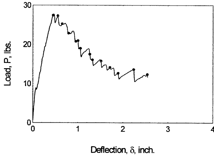
Figure 19: Load-displacement plot of regular DCB 93-oz specimen (No. 1) at constant displacement rate.
