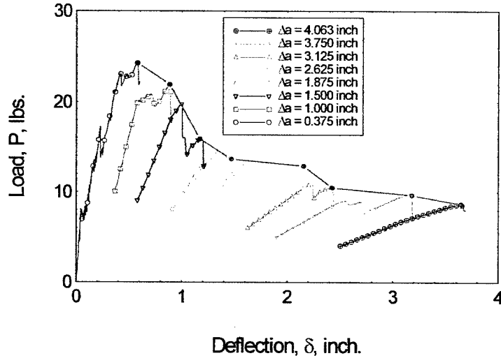
Figure 20: Load-displacement plot of regular DCB 93-oz specimen (No. 2) with unloading and reloading at different crack extension.
