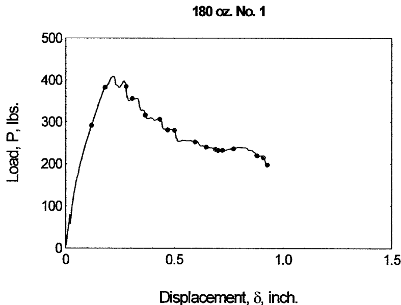
Figure 24: Load-displacement plot of tabbed DCB 180-oz specimen (3Weave™ #5 specimen 1) at constant displacement rate.
