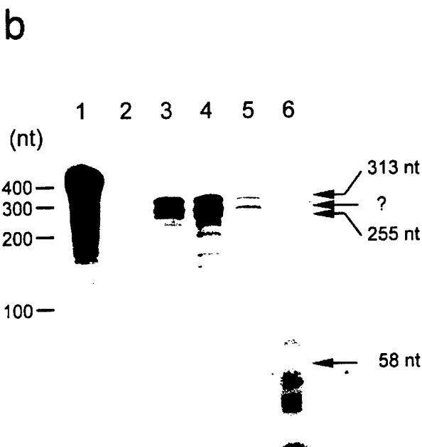
Figure 2. a) Schematic representation of antisense RNA probe used for RNase protection assay. The expected protected fragments from BRCA2 and BRCA2a transcripts are shown. b) Analysis of the expression of BRCA2a in different human tissues by RNase protection assay. This assay was carried out on 20 \mu g of total RNA using Ambion RPA kit. Lane 1, probe; Lane 2, tRNA; Lane 3, thymus; Lane 4, testis; Lane 5 mammary gland; Lane 6, prostate. Lanes 1-4 are the result of short exposure (1 day) and lanes 5 and 6 are of longer exposure (3 days). Protected 313 nucleotides (corresponding to the alternatively spliced BRCA2a) and 255 and 58 nucleotide fragments (corresponding to the BRCA2) are shown by arrows.
