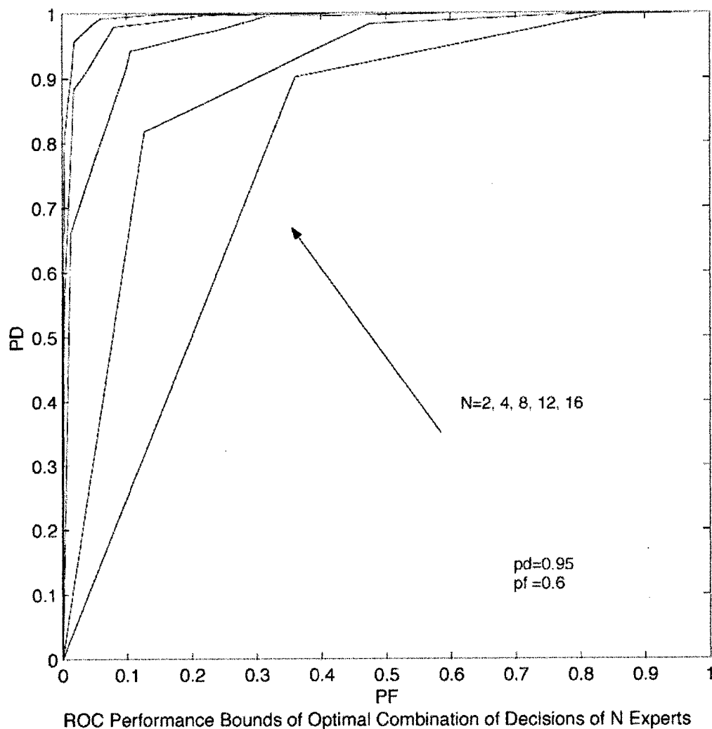
Fig. 6 illustrates the upper bound ROC for optimally combining the outputs of N experts, if each expert is operating at a sensitivity (TPF) of 0.95 and a false positive fraction (FPF) of 0.60.
