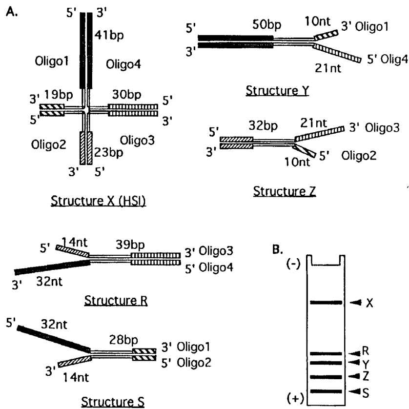
Figure 3. Schematic diagrams of predicted hybrids (A) and their relative mobilities (B). Five possible hybrids can form from a mixture of the four oligonucleotides. One will be HS. HS has four different lengths of arms (41, 30, 23 and 19bp). Other hybrids will be partial duplex DNAs annealed from the complementary sequences of Oligo3 and Oligo4, Oligo1 and Oligo2, Oligo1 and Oligo4, and Oligo2 and Oligo3. These structures are identified as R, S, Y and Z. R, S, Y and Z have different double-stranded portions of 39, 28, 50 and 32bp with two single-stranded tails, respectively. All of these hybrids have different sizes and degrees of double-stranded character, and all can be separated by their electrophoretic mobilities. HS is the largest molecule and will have the slowest mobility, as illustrated in the panel B on a native polyacrylamide gel. S is the smallest and will have the fastest mobility. Filled boxes or cross-hatched represent the flanking sequences. Open boxes represent the 18nt central sequences. The relative proportion of the hybrids differs in the hybridization mixture, because the hybrids have different T_m s. We routinely detect only three hybrids, HS, Y and Z, as will be shown in Figure 4.
