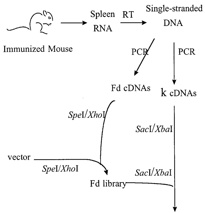
Figure 12. Construction of Fab expression library. The Fab expression library is derived from splenic RNAs. Briefly, total RNA will be isolated from spleens of HS-immunized mice. The RNAs will then be reverse transcribed into single-stranded DNA with Fd 3' and \kappa 3' priming. The single-stranded DNA will be used as templates for generation of IgG and IgE Fd and \kappa cDNA by PCR. The Fd and \kappa genes will be amplified separately with murine IgG primers, including one Fd 3' primer, nine Fd 5' primers, one \kappa 3' primer and five \kappa 5' primers (Huse et al. , 1989). Each pair of primers will give rise to a product of about 700bp. All the primers contain a restriction enzyme site: the Fd 3' primer has a SpeI site, the Fd 5' primer an XhoI site, the \kappa 3' primer an XbaI site, and the \kappa 5' primer a SacI site. These enzyme sites allow the double-stranded PCR products to be cloned into an Fab overexpression plasmid vector. This vector features a single bacteriophage T3 promoter in front of the Fd and \kappa cDNAs. The PCR products will be digested by corresponding restriction enzymes and the DNA will be gel-purified. SpeI/XhoI -digested Fd cDNA will be ligated into the SpeI/XhoI sites of the vector
