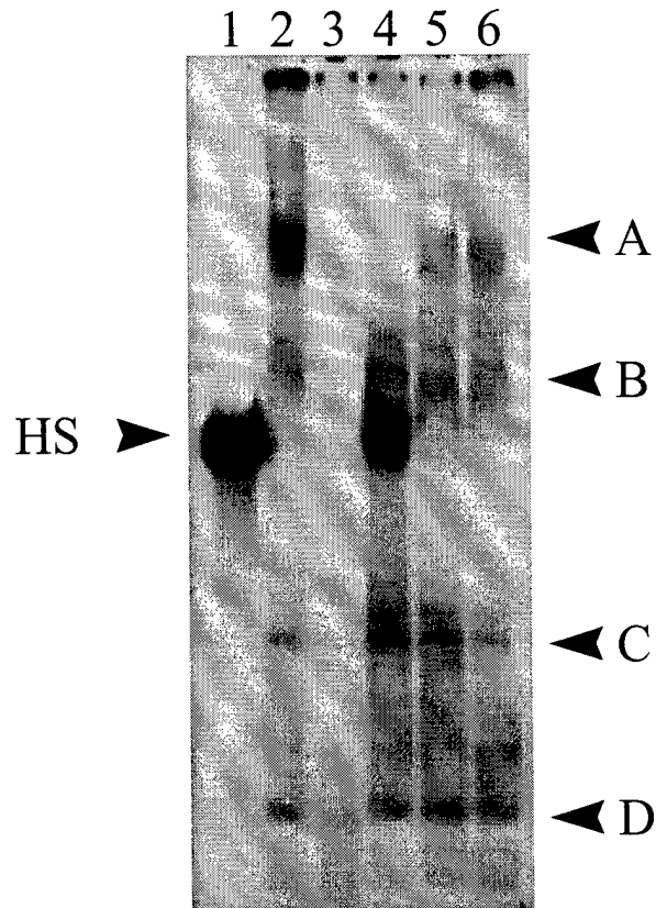
Figure 7. Binding specificity of antibodies to HS. The binding specificity of these proteins was tested, using serum from mouse 1. ( Note: This serum was taken after one more boost to the mouse and so was different from the mouse 1 serum used in Figure 6, lane 2.). All lanes contain equal amount of purified ^{32}\text{P} -labeled HS and were incubated with: lane 1, buffer alone; lanes 2, mouse 1 anti-serum (1:20) only; lanes 3-6, both mouse 1 serum (1:20) and goat anti-mouse IgG, purified non-labeled HS (30x in molar excess), Y (100x) and Z (100x), respectively. In the presence of the anti-serum, ^{32}\text{P} -labeled HS was distributed into four major entities, designated A, B, C, and D (lane 2). Addition of goat anti-mouse IgG blocked the formation of A and B (lane 3). This blockage indicates that A and B are HS-antibody complexes. A could be displaced by addition of a 30-fold molar excess of non-labeled HS (lane 4). However, addition of a 100-fold molar excess of Y or Z had no effect (lane 5 and 6, respectively). The results indicate that the antibodies are saturable and bind specifically to the central structure of HS. The electrophoretic mobilities of C and D were unaltered by addition of any competitor. Since both C and D have greater electrophoretic mobilities than the probe (HS), we doubt that these are DNA-protein complexes. Finally, the electrophoretic mobilities of C and D are different from those of the dimeric hybrids that we have called Y and Z (Figure 4). Although the identity of C and D remains to be established, the electrophoretic mobility of these two entities is consistent with the hypothesis that they represent a pair of resolved, double-stranded products of an antibody-catalyzed integrase reaction. We therefore conclude that some of the antibodies in the serum may possess integrase activity. The assay condition is as described in Figure 6 legend. Double-stranded DNA was annealed by mixing stoichiometric amount of the appropriate oligonucleotides in TE buffer.
