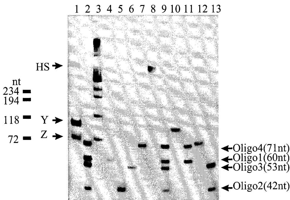
Figure 4. Formation and characterization of HS. Lane 3 is a set of ^{32}\text{P} -labeled single-stranded molecular size markers derived by denaturing Hae III digested bacteriophage phiX174 DNA. Lanes 4 through 7 contain ^{32}\text{P} -labeled oligonucleotides Oligo1 (60nt), Oligo2 (42nt), Oligo3 (53nt), and Oligo4 (71nt), respectively. The four ^{32}\text{P} -labeled oligonucleotides have different sizes and can be distinguished by their electrophoretic mobilities on the gel. The smallest one, Oligo2 (42nt), has the fastest mobility (lane 5); and the biggest one, Oligo4 (71nt) has the slowest (lane 7). Stoichiometric amounts of the four oligonucleotides were mixed in TE buffer (10mM Tris-HCl, pH8.0, 1mM \text{Na}_2\text{EDTA} ) (Duckett et al. , 1988), denatured at 100^\circ\text{C} for 5 minutes, incubated at 65^\circ\text{C} for 2 hours and allowed to cool slowly to room temperature. The mixture is resolved into three major entities, HS, Y, and Z (lane 1). This mixture of HS, Y, and Z was heat-denatured in urea to show that the mixture contained the four individual oligonucleotides (lane 2). The hybrids were purified by eluting the corresponding bands from a native 5% preparative polyacrylamide gel, with recovery by ethanol precipitation. Lanes 8, 10 and 12 are purified hybrids HS, Y and Z, respectively. Lanes 9, 11 and 13 are the denatured hybrids, respectively. Since HS has the slowest electrophoretic mobility and dissociates into a stoichiometric mixture of all four labeled component oligonucleotides, Oligo1, Oligo2, Oligo3 and Oligo4, as shown in lane 9, we assumed that HS is a Holliday structure. The mixture, or the oligonucleotides or the marker were labeled by \gamma - ^{32}\text{P} -ATP at their 5'-ends by T4 polynucleotide kinase according to Ausubel et al. (1987a). The denaturation was carried out by heating the samples in 5M urea at 95^\circ\text{C} for 3 minutes. Non-denatured samples were mixed with one fifth volume of loading buffer (50% [v/v] glycerol, 0.025% [w/v] xylene cyanol, and 0.025% [w/v] bromphenol blue). All the samples were then loaded on a 7% native polyacrylamide gel electrophoresed in 1 X TBE buffer (100mM Tris, 2mM \text{Na}_2\text{EDTA} , 100mM boric acid). After electrophoresis the gel was dried and exposed to X-ray film.
