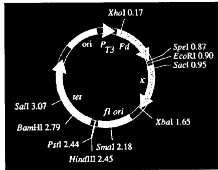
Figure 12. Construction of Fab expression library. The Fab expression library is derived from splenic RNAs. Briefly, total RNA will be isolated from spleens of HS-immunized mice. The RNAs will then be reverse transcribed into single-stranded DNA with Fd 3' and \kappa 3' priming. The single-stranded DNA will be used as templates for generation of IgG and IgE Fd and \kappa cDNA by PCR. The Fd and \kappa genes will be amplified separately with murine IgG primers, including one Fd 3' primer, nine Fd 5' primers, one \kappa 3' primer and five \kappa 5' primers (Huse et al. , 1989). Each pair of primers will give rise to a product of about 700bp. All the primers contain a restriction enzyme site: the Fd 3' primer has a SpeI site, the Fd 5' primer an XhoI site, the \kappa 3' primer an XbaI site, and the \kappa 5' primer a SacI site. These enzyme sites allow the double-stranded PCR products to be cloned into an Fab overexpression plasmid vector. This vector features a single bacteriophage T3 promoter in front of the Fd and \kappa cDNAs. The PCR products will be digested by corresponding restriction enzymes and the DNA will be gel-purified. SpeI/XhoI -digested Fd cDNA will be ligated into the SpeI/XhoI sites of the vector
