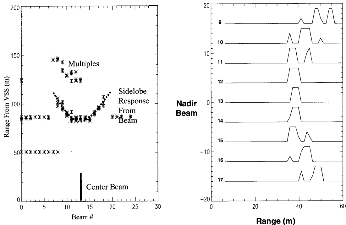
Figure 3 Recorded bottom return and multiples from a single VSS acoustic ping. Dark (*) is higher intensity acoustic return than lighter (*). Right side shows the 2-bit amplitude detection on each beam.
