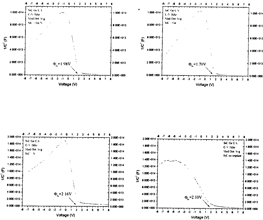
Figure 6. Capacitance-Voltage measurements made of SiC, n-type SiC, SiC:Ge, and n-type SiC:Ge showing varying built in voltages and a minimum value of built in voltage for the SiC:Ge sample.
