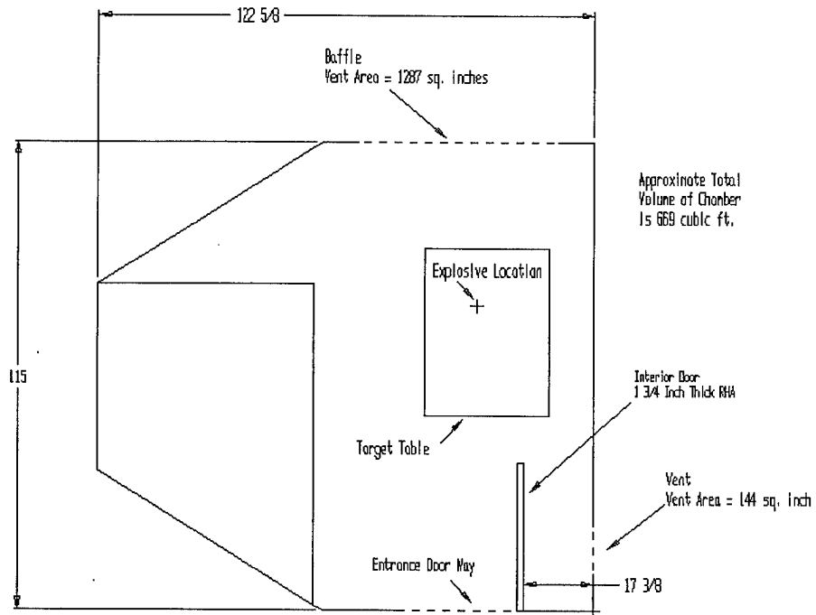
Figure 5. Schematic of Experimental Facility 108 A/B chamber.
