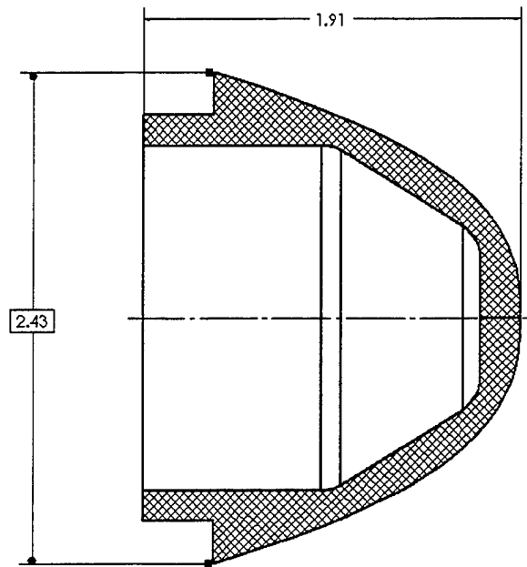
Figure 3. Hemispherical Radome Geometry (units in inches).
