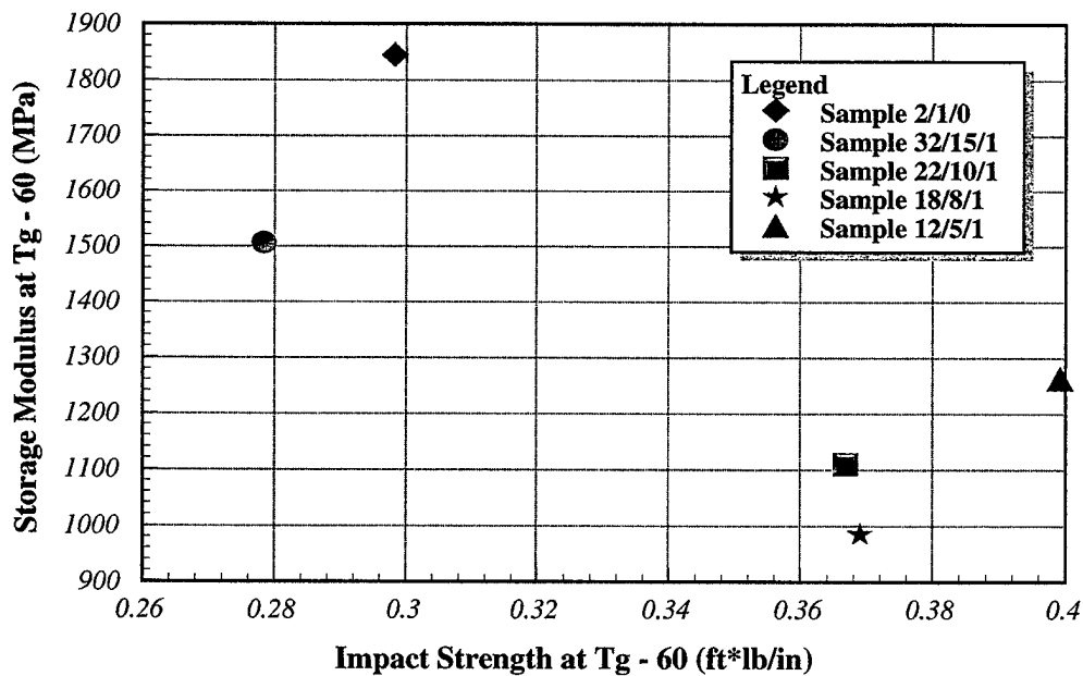
Figure 28. Storage Modulus Versus Impact Strength at T g - 60°C. (Notice the scatter in this figure. The storage modulus should decrease with increasing impact strength; apparently this is not the case for the 12/5/1 sample.)
