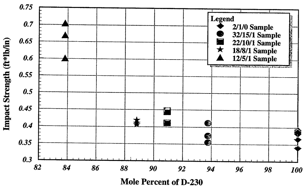
Figure 10. Impact Strength Versus Mole Percent D-230 at -180^{\circ}\text{C} . (Notice the decrease in impact strength from those at room temperature, except for the 12/5/1 sample, which did not change.)
