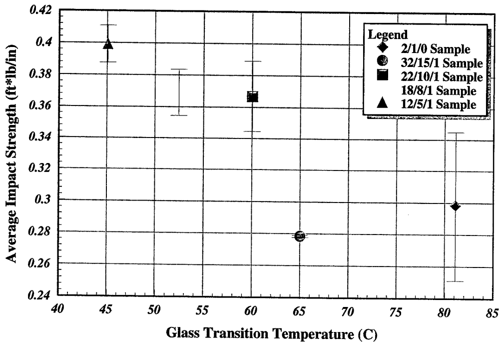
Figure 18. Average Impact Strength Versus Glass Transition Temperature at 60°C Below T_g With Error. (Again it follows the same trend as Figures 9 through 14.)
