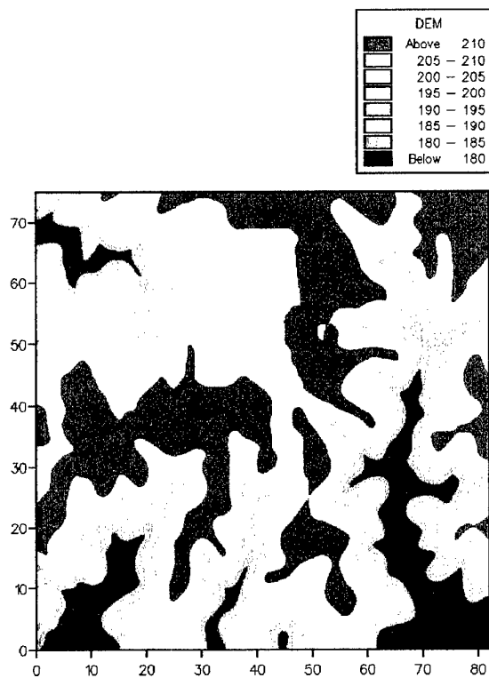
Figure 12. Map of punctually kriged estimates of elevation using the stable exponential model for 'aphillcut'.
