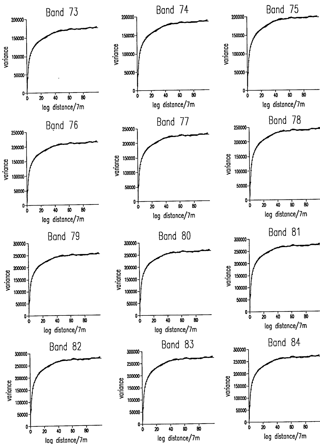
Figure 38: Experimental; variograms (symbols) and fitted models (lines) for bands 73 to 84
