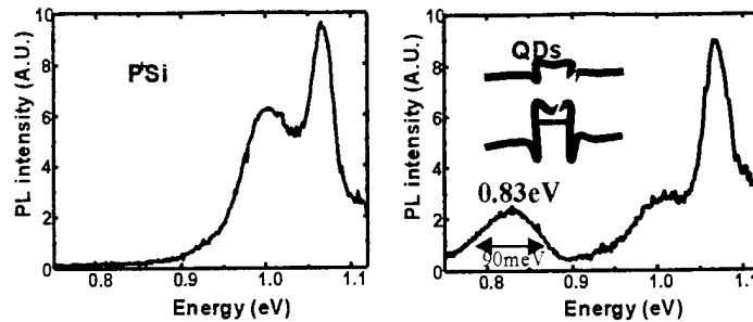
Spatially type II transition From ground state to Si CB edge ~330meV FWHM ~90meV (size distribution)
